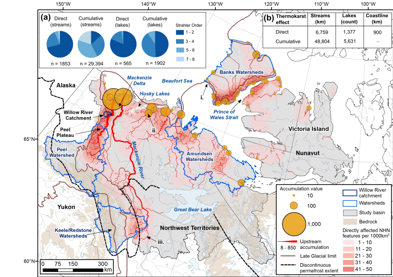
Figure 8. Thaw-driven landslide density and downstream accumulation of effects, western Canadian Arctic drainage from continuous permafrost terrain. Heat map depicts all directly affected stream, lake and coastal hydrological features mapped. All upstream accumulation values shown within the fluvial network are >2 and at the coast are >9. Accumulated effect contributions of the Mackenzie and Peel Rivers to the Beaufort Sea are routed separately for comparison. (a) Counts of direct and accumulated thaw-driven mass wasting 650 effects to fluvial systems partitioned by Strahler order and hydrological feature type for the four major watersheds outlined in blue. (b) Table showing lengths of directly affected hydrological network and accumulated effects, count of directly and indirectly affected lakes and total directly affected coastline for western Arctic drainage from continuous permafrost. Remote sensing examples of thaw-driven downstream sedimentation provided in Fig. S4 for: i) Sachs River and Fish Lake, ii) Miner River inflow to the Husky Lakes estuary and 655 iii) massive deep-seated permafrost failure on Johnson River. Late glacial limit is from Dyke and Prest, 1987, bedrock geology is from Fulton, 1995, and the permafrost boundary is from Brown et al., 1997. Base map is from ESRI ArcGIS Online.
