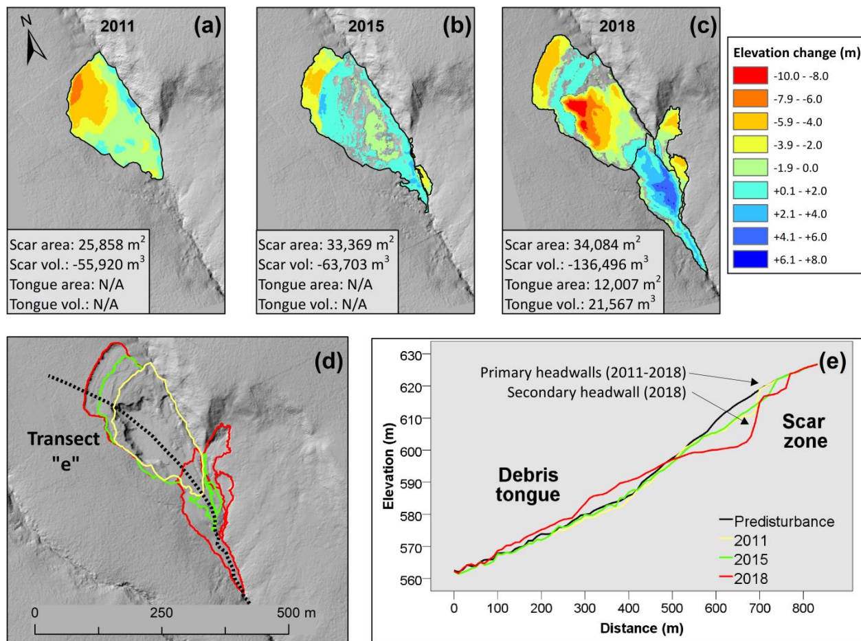
Figure 3. Thaw slump growth (slump CB), material displacement and evolution of downstream connectivity 2011 to 2018, Peel Plateau, Northwest Territories, Canada. (a) 2011 difference from the reconstructed pre-disturbance terrain surface; (b) 2015 terrain differenced from the 2011 terrain; (c) 2018 terrain differenced from the 2015 terrain, showing polycyclic behaviour including thaw-driven evacuation of scar materials, and development of a prominent lower “secondary” headwall and scar concavity. Slump and debris tongue area and volumes are calculated relative to estimated pre-disturbance surface. (d) The evolution of thaw slump footprint from 2011 to 2018 and the topographic transect in (e) showing elevation profiles through the slump and along the valley for pre-disturbed terrain, 2011, 2015 and 2018. Hill-shade in (d) is the 2018 UAV survey integrated with the surrounding 2011 regional LiDAR data.
