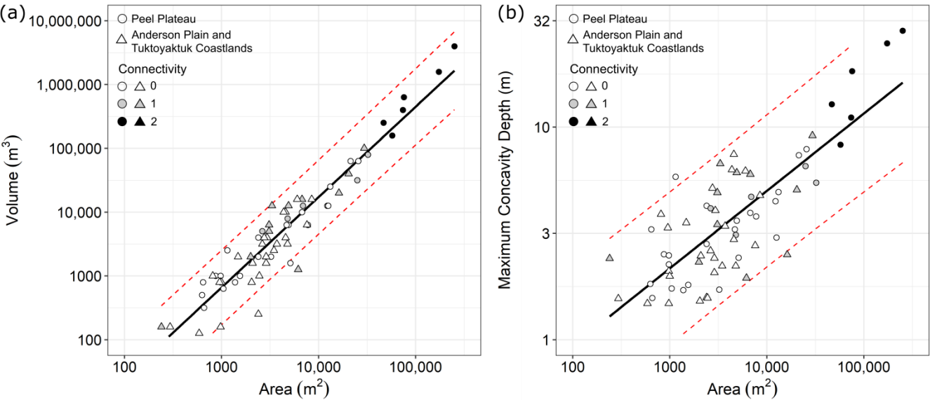
480 Figure 4. Relationships between: (a) slump scar area and volume ( R^2 = 0.90 ; F=641.9 ; N=71 ; P<0.0001 ), and (b) slump scar area and maximum depth of concavity ( R^2 = 0.63 ; F=116.2 ; N=71 ; P<0.0001 ) for disturbances in the fluvially-incised Peel Plateau, and lake dominated Anderson Plain/Tuktoyaktuk Coastlands. Connectivity between slope and downstream environment is categorized by: 0) no connectivity; 1) physical connection between bare scar and downstream environment; and 2) evidence of downstream deposition of materials into valley, stream channel or lake. Red dashed lines show 95% confidence limit. Regression diagnostics indicate that residuals are normally distributed and there are no unduly influential points.
