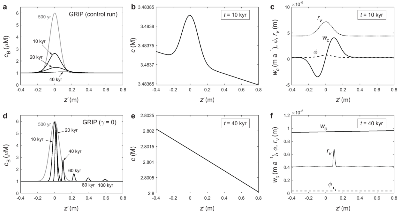
Figure 5: Modelled evolution of a signal peak in (a–c) the GRIP control run and (d–f) an otherwise identical run where the Gibbs–Thomson effect is turned off ( \gamma = 0 ). Snapshots are shown in the material reference frame, with displacement z' measuring how far the signal has moved from ice of the same age (which lies at z' = 0 ). (a,d) bulk solute concentration c_B ; (b,e) vein solute concentration c at one time; (c,f) anomalous velocity w_c , porosity \phi , vein curvature r_v at one time. Grey curves in (a) and (d) indicate the initial doped peak. Panel b illustrates the Gibbs–Thomson perturbation. See Movie S1 for the full simulations.
