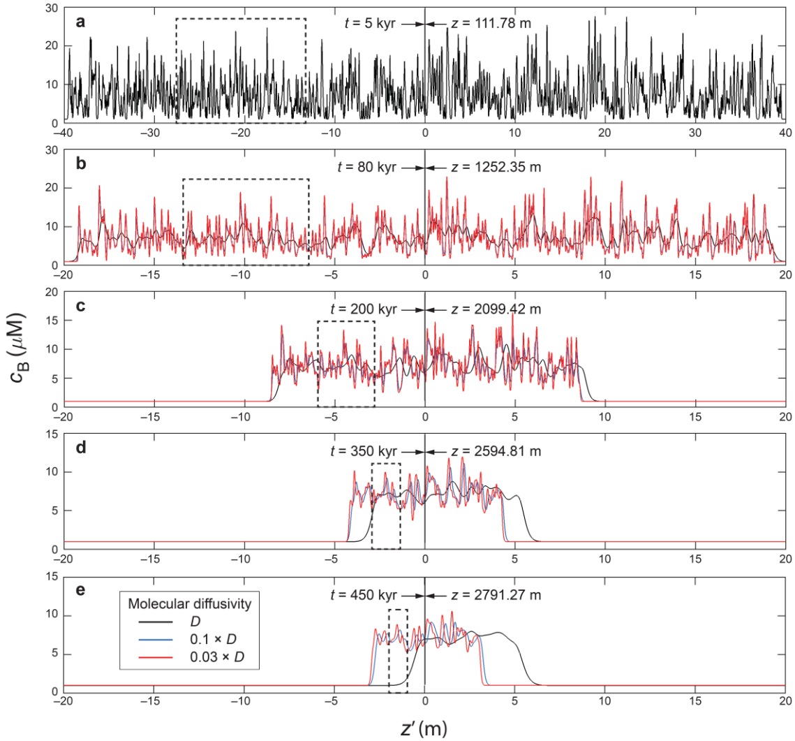
1065 Figure 11: Simulated evolution of a long sequence of doped signals at the EPICA site, in three experiments assuming the molecular diffusivities D (Table 1), 0.1D and 0.03D . (a) Initial c_B sequence. Used in all three runs and made from the superposition of 1200 decimetre- scale Gaussian peaks, it is not meant to recreate the actual signals at EPICA. (b)–(e) Snapshots of c_B at later times. Labels near the vertical line indicate the depth and age of the ice at z' = 0 . The dashed boxes trace a group of signals as they evolve into new signals through compression-diffusion merging (Sect. 3.3). As D is reduced, signal persistence into deep ice improves, and signal displacement decreases. 1070 The duration of the signal sequence is \approx 3,600 yr in all panels. See Movie S5 for the full simulations.
