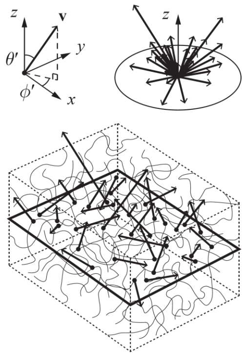
Figure B1: Velocities \mathbf{v} of different vein segments crossing a plane (outlined by bold rectangle), and their distribution in spherical coordinates (upper right). Only crossings in one direction are shown. In Appendix B, a statistical theory is used to calculate the net transport of porosity and vein impurity resulting from this motion.
