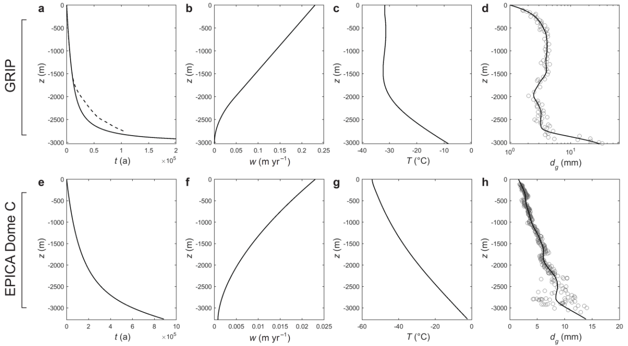
925 Figure 4: Ice-core background fields used in our signal evolution experiments. GRIP ice core: a to d. (a) Age-depth scale and (b) ice velocity from a Dansgaard-Johnsen model. Dashed line in (a) shows the GICC05 model ext time scale (Seierstad et al., 2014; Rasmussen et al., 2014). (c) Ice temperature from Johnsen et al. (1995). (d) Grain-size data from Thorsteinsson et al. (1997) and spline fit used in our modelling. EPICA Dome C core: e to h. (e) Age-depth scale and (f) ice velocity from the model described in Sect. 3.1. (g) Borehole temperature from Pol et al. (2010). (h) Grain-size data from Durand et al. (2004) and spline fit used in our modelling.
