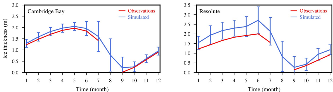
Fig. 1. Figure 1. Seasonal variability of the sea ice thickness from CIS (red curve) and AO-FVCOM (blue curves) over the period 1979–2017.
