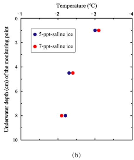
Figure 6. Monitoring of the through-thickness thermal gradient of floating ice: (a) a schematic diagram of the arrangement of the temperature probes and (b) the measured through-thickness thermal gradient inside two floating ice specimens.
