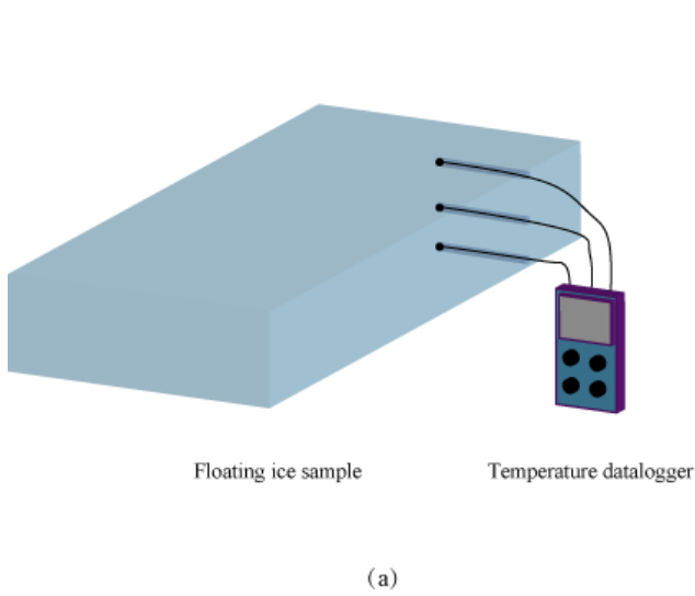
Figure 6. Monitoring of the through-thickness thermal gradient of floating ice: (a) a schematic diagram of the arrangement of the temperature probes and (b) the measured through-thickness thermal gradient inside two floating ice specimens.
