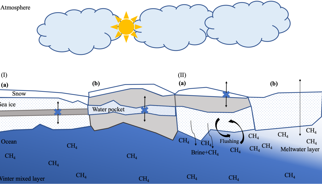
Figure 5: Potential pathways of methane in sea ice with varying impermeable (indicated in grey) and permeable sections (in white with blue dots), i.e. winter (I) and spring (II) conditions. I (a) Relicts of the initial methane signal (source) entrapped in impermeable ice layers. Impermeable intermediate sea ice layers, act as a barrier for the upward/downward transport of methane (black arrow overlaid by a blue cross). (b) Residual methane signal after methane oxidation occurred in permeable sea ice layers (“water pocket”), enclosed by impermeable ice layers (see Fig. 6). II (a) When basal melt starts, but the top layer still is impermeable and with snow cover (white layer on top of the ice), downward brine transport initiates release of dissolved methane. Flushing events trigger methane released into the ocean (see chapter 4.1.3). (b) Un-restricted migration of methane in permeable sea ice layers (black dotted arrow). Ongoing sea ice melt, when freshwater from melted sea ice is released into the water underneath, resulting on a meltwater layer, where methane remains sustained during late spring. Methane ( \text{CH}_4 ) annotation indicates concentration. Color gradient in the ocean, reflects the increasing stratification during the seasonal evolution of the upper part of the WML (in blue) into a fresh meltwater layer (in white).
