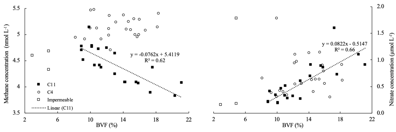
Figure 7: (a) Methane and (b) nitrate concentration vs. brine volume fraction (BVF) at C11 and C4, respectively. In C11, methane is inversely correlated ( R^2=0.62 ) while nitrate is correlated ( R^2=0.66 ) with increasing BVF. This trend shows that methane is released from ice while nitrate is taken up. In station C4, correlation is missing when sea ice is fully permeable. C4 shows an homogenous distribution of methane as well as nitrate, and higher concentration than in C11, caused by flushing of seawater charged in methane and nitrate into the sea ice. The three outliers points (impermeable ice layers) have been removed for the correlations.
