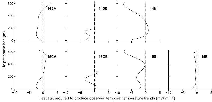
Figure 4: Additional heat fluxes required to maintain observed rates of temperature change if the collected static temperature profiles diffusionally evolve over time evolve through vertical thermal conduction over time. Dashed line indicates the switch between a required heat source or sink.
