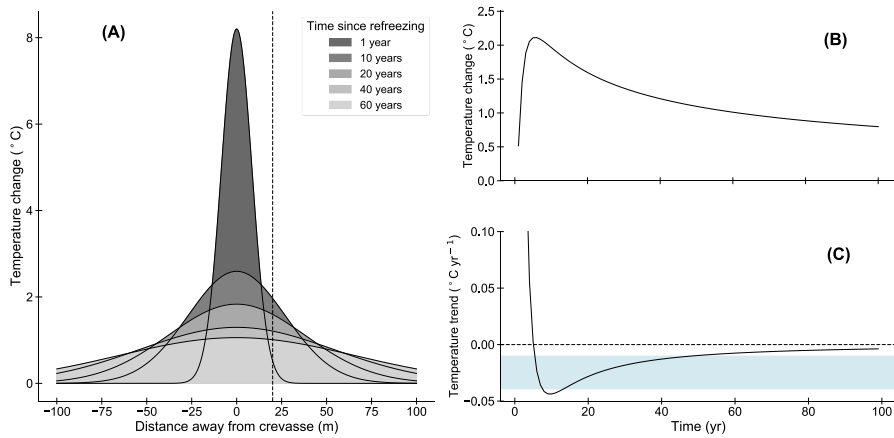
530 Figure 6: (A) Modeled changes in temperature after a crevasse 1 m wide refreezes. Darker colors show earlier times. Dashed line indicates a distance 20 m from the crevasse, which temperatures and temporal rates of temperature change are shown in B and C. (B) Changes in temperature over time at 20 m away from the basal crevasse. (C) Corresponding rates of temperature change for panel B. The blue shaded region shows the range of averaged rates of cooling in the lowest 100 m of the boreholes.
