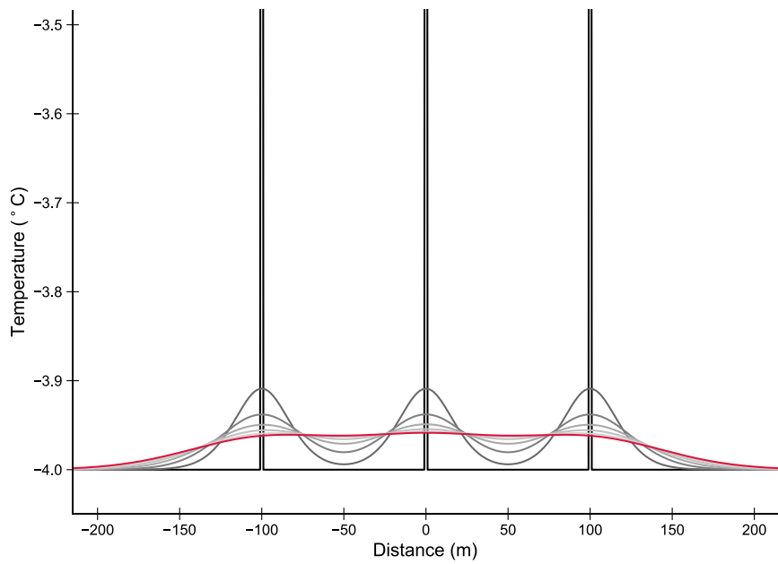
Figure 7: Evolution of a synthetic 1-D temperature field from basal crevasses spaced 100 m apart. Temperatures are plotted every 5 years, and older temperature fields are shaded darker shades of grey. Red line shows the temperature field 30 years after refreezing. Distinct crevasses can cause cooling over large regions of the bed.
