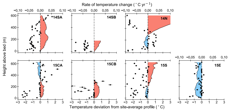
Figure 5: Rates of temperature change for each borehole (black dots) plotted with temperature deviations from the best-fit profile at each borehole within each borehole from the site-average temperature profile. Red shaded regions indicate that the collected static profile is warmer than a pure diffusion profile the site-average profile, and blue shaded regions show the static profile is colder than the diffusion profile site-average profile. Error bars on the calculated rates are the same as in Fig. 3. Only boreholes that have full-depth data are shown.
