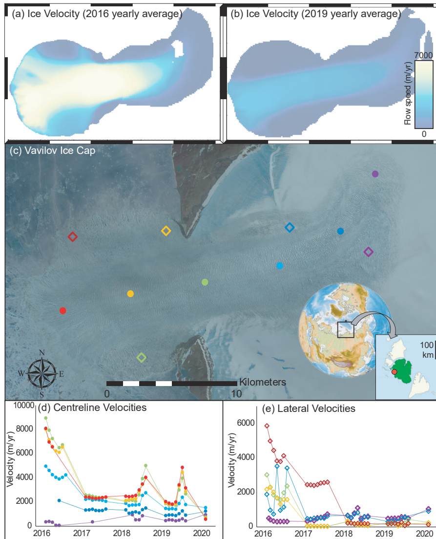
Figure 8. (a) and (b) 100-m-resolution annual mean velocities for the western outlet glacier of Vavilov Ice Cap. (c) a 2019 Sentinel-2 image showing the main features of this outlet and the locations used to derive monthly timeseries. (d) and (e) monthly resolution velocity timeseries along the glacier centreline and flanks using Sentinel-2 imagery.
