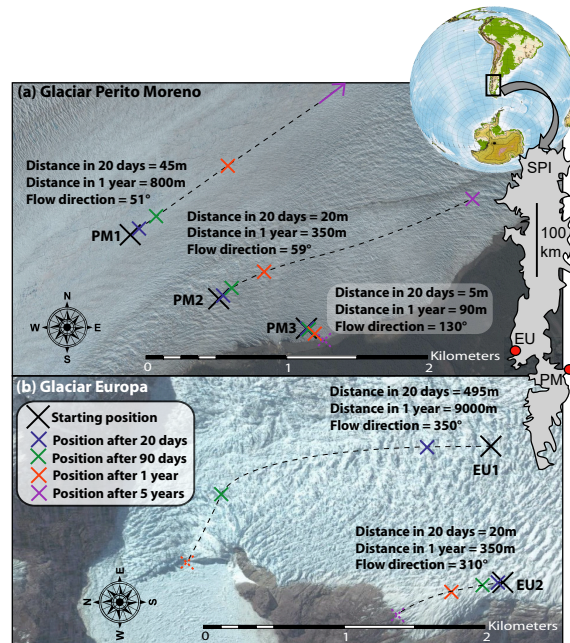
Figure 6. (a) Position of a point on Glaciar Perito Moreno (PM) with time for three different starting locations within 2 km of the glacier’s southern margin. At PM1, ice speeds reach 800 m/yr and any equipment will be rapidly displaced. At PM3 ice-flow speeds are < 100 m per year and oriented towards the valley edge. (b) Identical plot for two points on Glaciar Europa (EU). Any equipment installed at EU1 will be displaced several kilometres and lost to calving in less than 6 months. The inlay shows an outline of the Southern Patagonian Icefield (SPI), with the locations of the two glaciers. Imagery © Google Earth.
