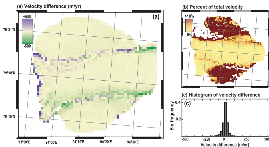
Figure 9. Comparison between Zheng et al. (2019b)'s velocity maps for Vavilov Ice Cap (Pair037_20170506_20170522) with results from GIV (May 2017 average). a) Difference map, corresponding to Zheng et al. velocity minus GIV velocity, b) percentage of the total velocity this difference represents (absolute value of the difference shown in a) divided by GIV velocity), and c) histogram of the difference values. The mean difference between the two velocity maps is less than 20 m per year, or less than 1% of the total velocity for much of the area.
