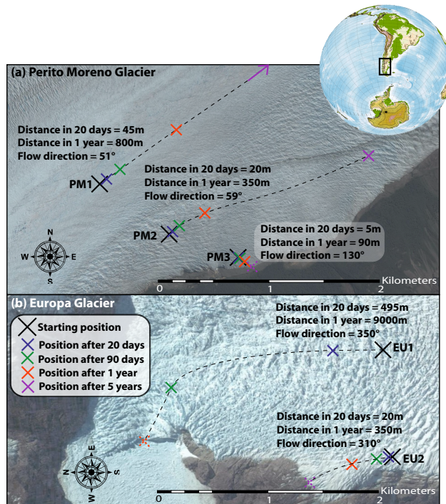
Figure 6. (a) Position of a point on Glacier Perito Moreno with time for three different starting locations within 2 km of the glacier's southern margin. At PM1, ice speeds reach 800 m/yr and any equipment will be rapidly displaced. At PM3 ice-flow speeds are < 100 m per year and oriented towards the valley edge. (b) Identical plot for two points on Glacier Europa. Any equipment installed at EU1 will be displaced several kilometres and lost to calving in less than 6 months. Imagery © Google Earth.
