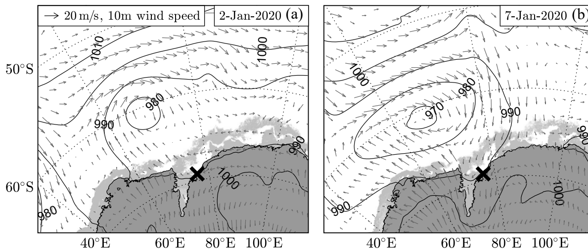
Figure 2. Passage of two storms offshore of the Antarctic instrument site on (a) 2-Jan-2020 and (b) 7-Jan-2020. Contours show mean sea level pressure, and wind speed at 10 m is displayed through the vector field (both from ERA5). Light gray shading represents sea ice, derived from AMSR2 data (Spren et al., 2008). The black cross identifies the deployment site. The presence of relatively high wind speeds over the polynya region on 07-Jan-2020 is expected to generate wind waves at the deployment site.
