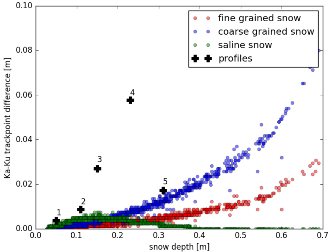
340 Figure 6. The Ka- and Ku-band track point difference as a function of snow depth (and density). The red points represent the profile in Table 1, while blue points represent coarse grained snow (correlation length: 0.3 mm) and green points represents saline snow (salinity 2 ppt). The five simulated profiles in Table 2 are marked with black crosses and the numbers refer to the profile number in Table 2.
