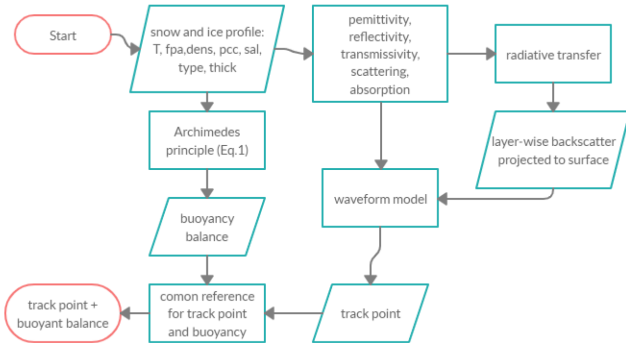
Figure 5. Computational steps in the scattering model to reach the radar altimeter track point. The model is described in detail in Tonboe et al., 2006a and 2010. The snow and ice profile has temperature (T), flat-patch-area (fpa), correlation length (pcc), salinity (sal), snow or ice type (type), and thickness (thick) for each layer.
