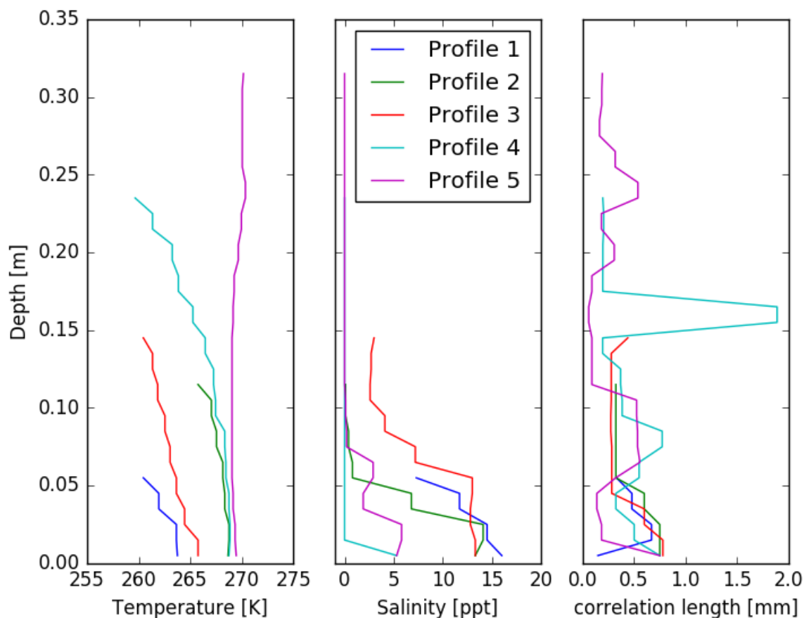
180 Figure 4. Snow temperature, salinity and snow grain correlation length of the 5 snow pit profiles on FYI, acquired from the Canadian Arctic. Depth = 0.00 corresponds to the bottom of the snow pack.
