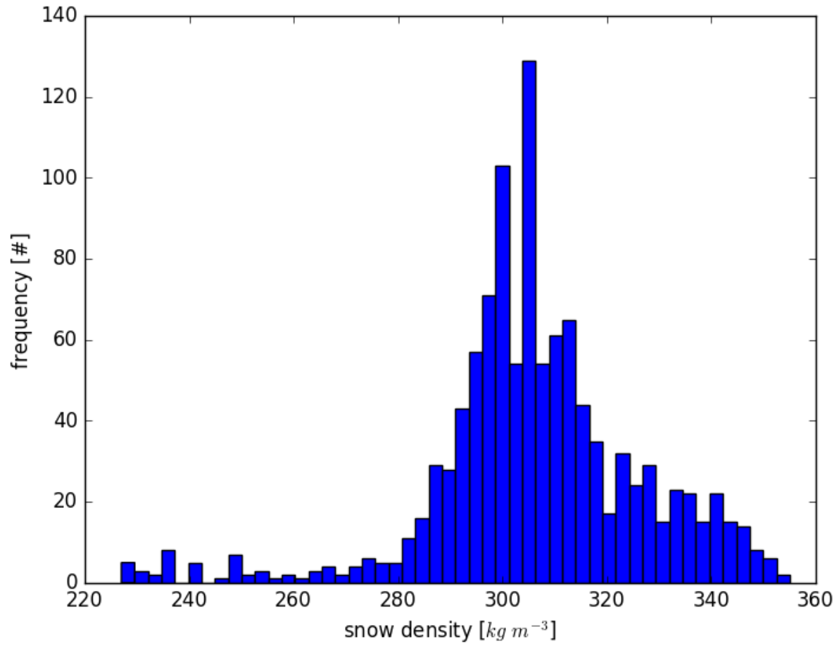
Figure 2. Snow density distribution (N=1114) in the RRD dataset (from W99 climatology) used as input to the scattering model. Mean snow density corresponding to March and April is 306 kg m -3 and the standard deviation is 20 kg m -3 .
