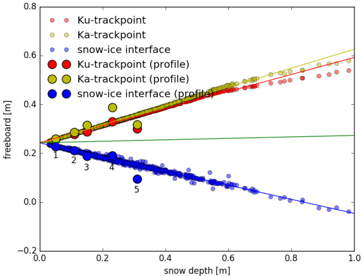
390 Figure 7. Red circles is the Ku-band radar track point as a function of snow depth and density, the linear fit (red line) is the freeboard, f_{Ku} = 0.35SnowDepth + 0.24 , yellow circles (and line) is the Ka-track point, f_{Ka} = 0.39SnowDepth + 0.24 , blue circles is the snow/ice interface freeboard as a function of snow depth and density, the linear fit (blue line) is 395 f = -0.29SnowDepth + 0.24 . The lines cross at a snow depth of 0.30 m (the physical meaning of the crossing point is related to the sea ice and sea water densities and the surface roughness and the radar frequency), the combined effect of the Ku-band track point and buoyancy is the green line freeboard, f = 0.03SnowDepth + 0.34 . The five snow profiles (numbers 1-5) from the Canadian Arctic are added, depicted with large blue circles for the snow/sea ice interface, large red and yellow circles for the Ka- and Ku-band track points, respectively (Table 2). (The figure is a reproduction of Fig. 3C in Tonboe et al. (2010) with new input data).
