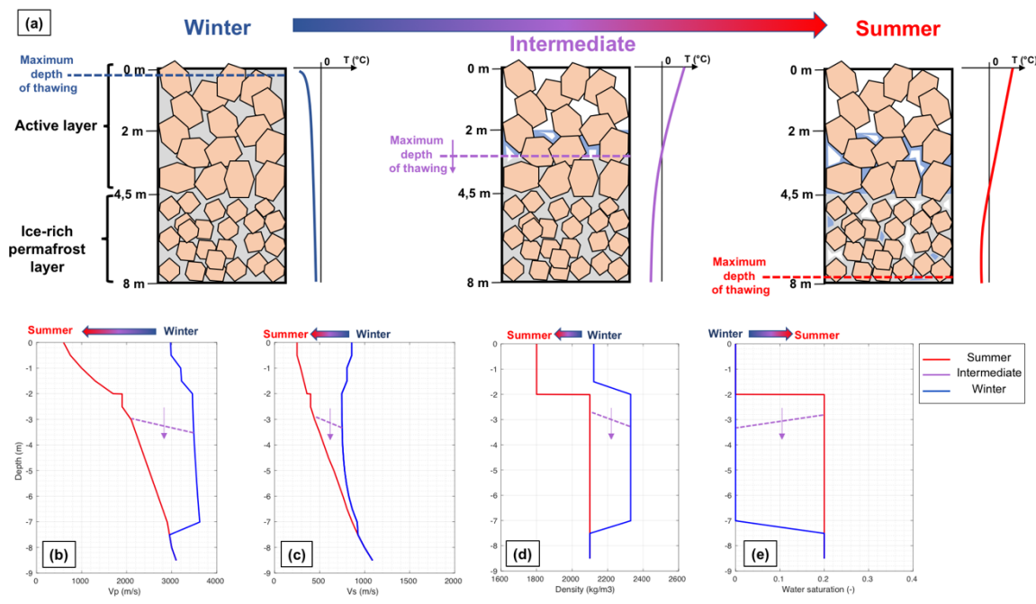
895 Figure 10: (a) Schematic cross-section of the Gugla rock glacier in winter (left) and in summer (right), and during the transition between them (intermediate state of thawing, in middle), as well as a schematic temperature profile associated with each of them, showing the main assumptions of the freezing modeling methodology by a poroelastic approach described in the text. The porous medium is composed of a rock matrix (in orange) and pores filled by water (in blue) or ice (in grey). With respect to the maximum depth of thawing varying from the surface to the ZAA depth, the evolution of parameters used by the model is respectively showed : P-wave velocity (b), S-wave velocity (c), the averaged density (d) and the water saturation (d). The 900 values in summer are obtained from geophysics and boreholes, whereas the values corresponding to a frozen state (pores fully filled by ice, no more liquid water) are obtained by the 3-phases poroelastic model.
