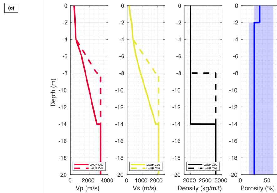
Figure 8 : (a) Cross-section of the Laurichard rock glacier Digital Elevation Models (DEM) of the surface and of the bed (taken for the bedrock) along the C05-C00 line. (b) The same profile, with the DEM of the surface as the reference. The vertical axis is then the bedrock depth starting from the surface. For both figures the location of the seismometers is indicated. (c) Seismic velocity models of the Laurichard rock glacier (continuous line for the C00 case, dashed line for the C05 case), based on geophysical investigations (seismic refraction) and the bedrock depth estimation, determined from DEM difference (see 1b). 885 The only difference between the two cases is the bedrock depth, and consequently the seismic velocity gradient of the
