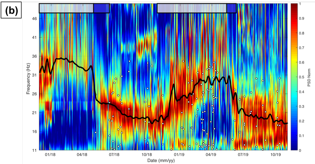
Figure 18: Normalized Power Spectra Density (PSD) from hourly spectrograms of the passive seismic recordings of Laurichard site, respectively from (a) C00 seismometer and from (b) C05 seismometer. The bold black line denotes the moving window average of hourly spectrogram maxima. For each recorded earthquake ( M > 2 ), the local maxima have been automatically picked (white dots) if it appears significantly on the spectrogram. Snow cover and melting periods are both figured by white and blue boxes above, respectively.
