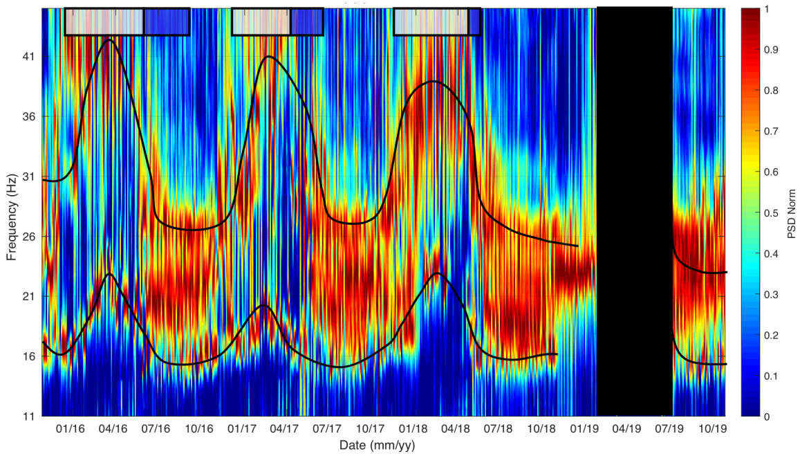
860 Figure 4 : Normalized Power Spectral Density (PSD) from hourly spectrograms of the ambient noise recordings of Gugla rock glacier, from C2 seismometer. Note the two bold black lines that roughly highlight the two picked spectral modes, for visibility purposes. Snow cover and melting periods are both figured by grey and blue boxes above, respectively. No-data period is marked by a black box.
