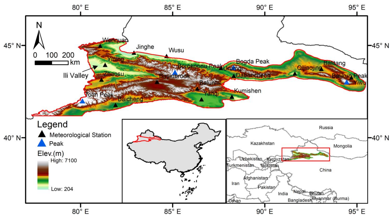
650 Figure 1: Location of the Chinese Tianshan Mountains (CTM). The elevation ranges from 204 m to 7100 m a.s.l., with a DEM resolution of 1 km from SRTM. The grey sub-plot show the extent of the CMA05 at the 0.5^{\circ} \times 0.5^{\circ} grid.
