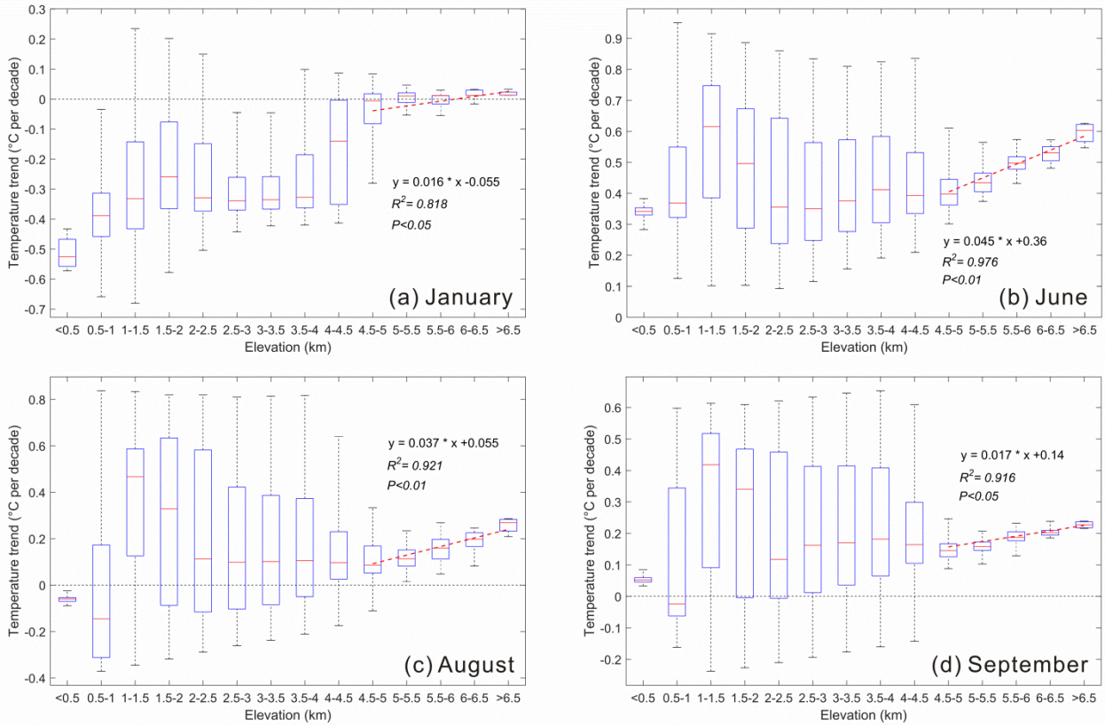
660 Figure 3: Box plots of monthly mean temperature trends at different altitudes from 1979 to 2016. (a) January, (b) June, (c) August, and (d) September. Thick horizontal lines in boxes show the median values. Boxes indicate the inner-quartile range (25% to 75%) and the whiskers show the full range of the values. The red dashed lines represent the significance of EDW by fitting the temperature trends and altitude groups above 4500 m.
