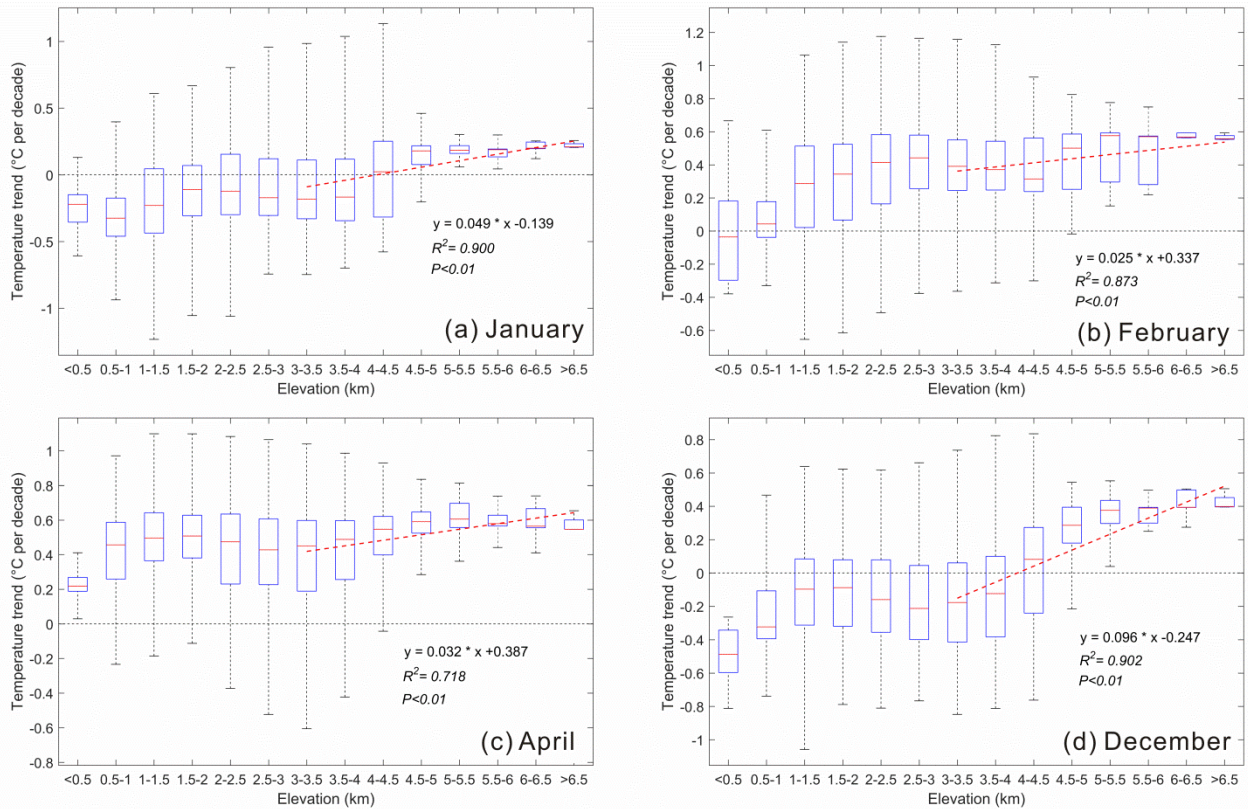
655 Figure 2: Box plots of monthly minimum temperature trends at different altitudes from 1979 to 2016. (a) January, (b) February, (c) April, and (d) December. Thick horizontal lines in boxes show the median values. Boxes indicate the inner-quartile range (25% to 75%) and the whiskers show the full range of the values. The red dashed lines represent the significance of EDW by fitting the temperature trends and altitude groups above 3000 m.
