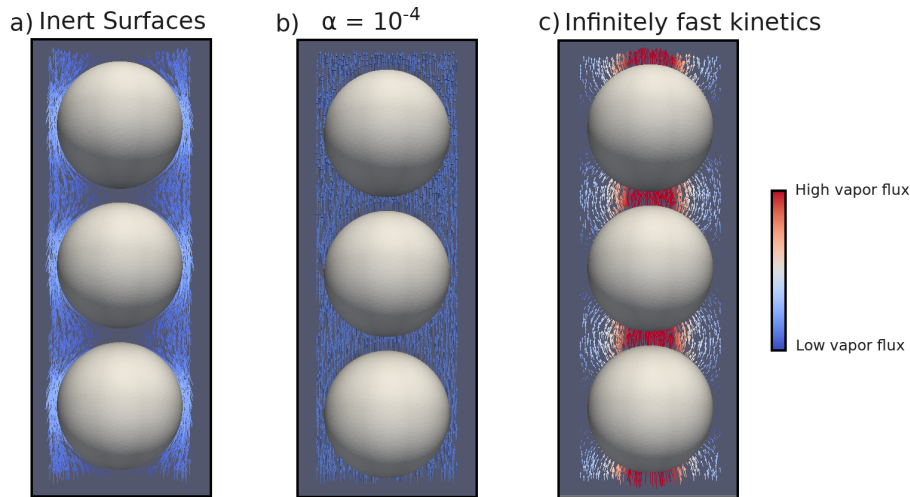
Figure 3. Disconnected ice spheres geometry with microscopic vapor fluxes in the pore space and for a 50 \text{ K m}^{-1} thermal gradient. a) Inert surfaces case, b) \alpha = 10^{-4} case, and c) infinitely fast kinetics case.
