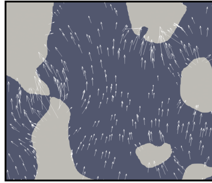
b) Infinitely Fast Kinetics
