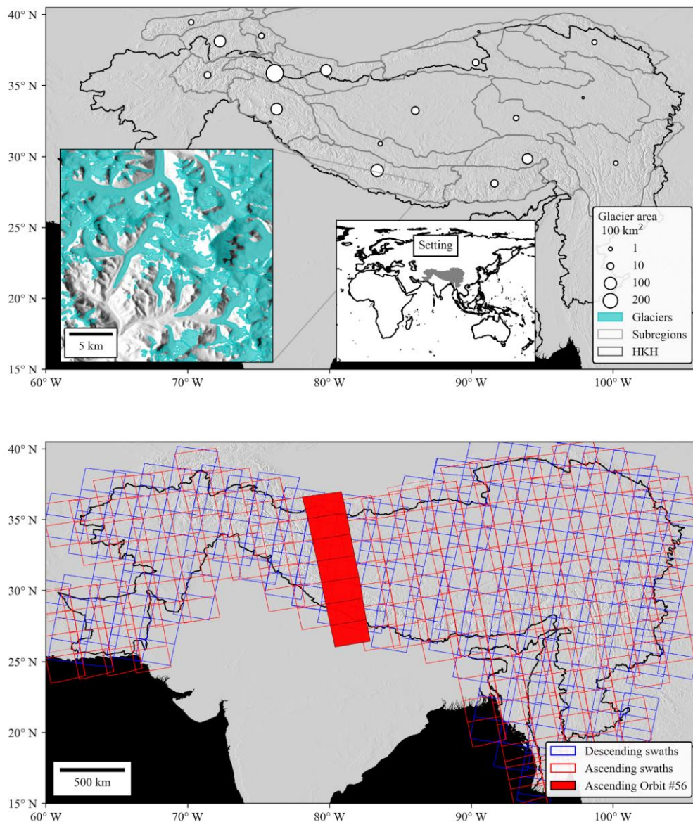
Figure 1. (Top) Hindu Kush Himalaya (HKH) region and 2018 GAMDAM glacierized areas summed across glacio-climate sub-regions from Shean, et al. (2020). An inset map highlights the spatial fidelity of GAMDAM outlines in the top panel. GGI and HKH data overlay a 30m Shuttle Radar Topography Mission (SRTM) DEM hillshade (Farr, 2007a). (Bottom) Sentinel-1 ascending (red) and descending (blue) swath footprints acquired across the study region. Ascending orbit cycle number 56 is highlighted in red to illustrate the SAR image processing approach for time series analysis across distinct orbit cycles.
