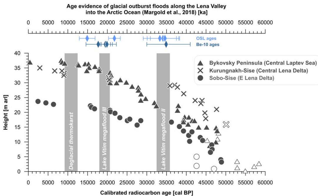
1160 Figure 12: Comparison of interpreted chronology gaps (shown as shaded rectangles) in the Yedoma IC records from Bykovsky Peninsula (Mamontovy Khayata; Schirrmeister et al., 2002a, 2011), Sobo-Sise Island (this study) and Kurungnakh-Sise Island (Schirrmeister et al., 2003; Wetterich et al., 2008a). Infinite radiocarbon dates or dates to be calibrated beyond the limit of 50 cal ka BP (Reimer et al., 2013) are minimum ages and given as hollow symbols. Age evidence from OSL and Be-10 dating for repeated megafloods (namely numbers II and III) from the glacial Lake Vitim along the Lena Valley into the Arctic Ocean (Margold et al., 2018) is shown for comparison.
