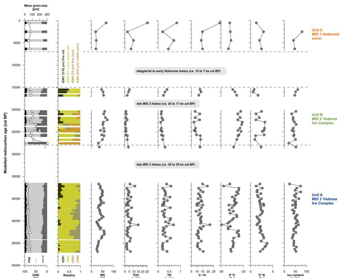
1130 Figure 5: Sediment properties of the Sobo-Sise Yedoma record and their variations over time. Dashed horizontal lines indicate the limits of the cryostratigraphic units A, B and C. White circles in the plot of grain-size properties relate to the upper x-axis (Mean grain-size).
