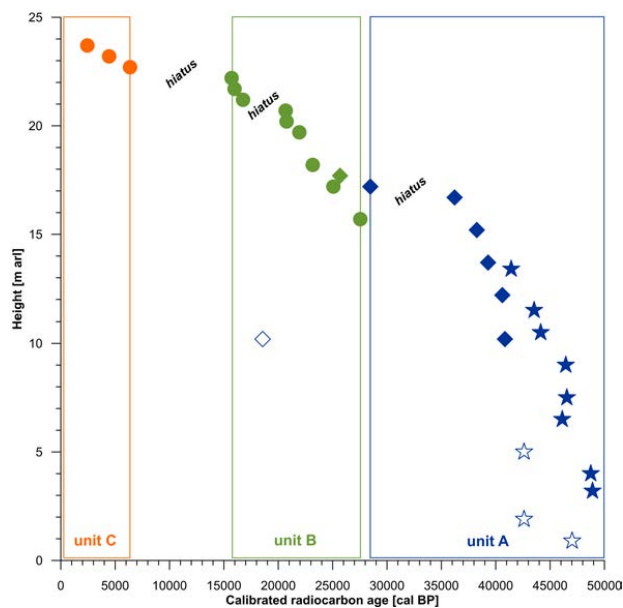
1125 Figure 4: Age-height relation of the Sobo-Sise Yedoma cliff exposure shown in calibrated radiocarbon ages. Note the sampling overlap of the profiles SOB18-01 (circles), SOB18-03 (diamonds) and SOB18-06 (stars) and their alignment to cryostratigraphic units A (blue), B (green) and C (orange). The open diamond indicates one age of redeposited material from sample SOB18-03-17 and open stars indicate infinite radiocarbon ages of samples from profile SOB18-06.
