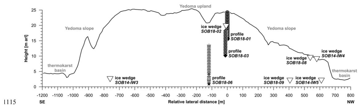
Figure 2: Profile positions of sediment profiles SOB18-01 (circles), SOB18-03 (diamonds) and SOB18-06 (stars) as well as ice-wedge profiles (triangles) sampled at the Sobo-Sise Yedoma cliff in 2014 (SOB14-...) and 2018 (SOB18-...). Cliff edge line elevation (relative to river level) was retrieved from ArcticDEM (10 m spatial resolution, Mosaic v3.0 10m: tile 59_43; Porter et al., 2018).
