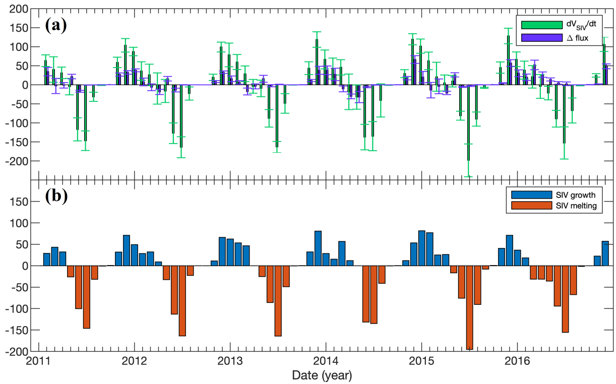
75 Figure 5. The ensemble mean sea ice volume changes from net ice flux and thermodynamics growth. (a) The ensemble mean SIV variability ( dV_{SIV}/dt , green bar) in the defined Baffin Bay area and the net SIV flux ( \Delta flux , purple bar) together with the ensemble spread (error bar). (b) The SIV variability derived from ice freezing (blue bar) and melting (orange bar) in the defined area.
