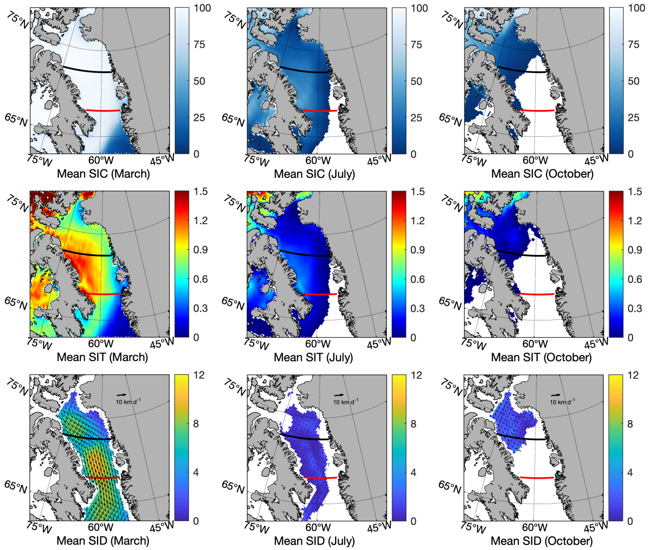
45 Figure 1. The ensemble mean sea ice concentration (top row: SIC, unit: %) and thickness (middle row: SIT, unit: m) in March, July, and October averaged from CMST, NAOSIM, PIOMAS and Sat-merged SIT over the period 2011-2016. Sea ice drift (bottom row: SID, unit: km d -1 ) is calculated by averaging data from NSIDC. Note that the Sat-merged SIT in the ensemble are only valid in March and October.
