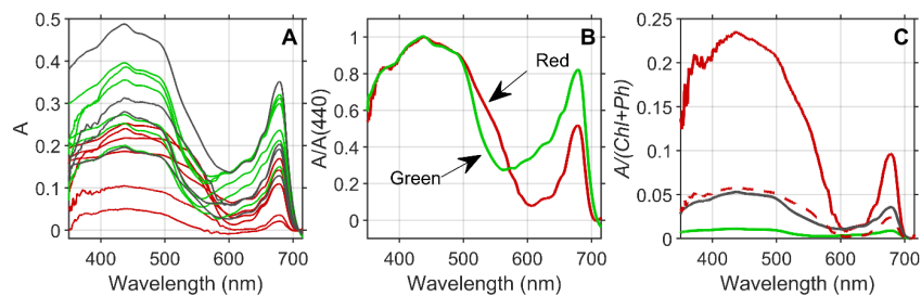
Figure 5. A) Estimated Absorbance ( A ) of the snow algae reveal distinct patterns of broad absorption in soiret or blue (400-500 nm) and a secondary peak in red wavelengths (678 nm) common to all algal groups, with green (green lines) and mixed (black lines) algae presenting higher absorption magnitude than red algae (red lines) due to enhanced pigment concentrations. B) The spectral shape of mean absorption normalized at 440 nm reveals that absorption by red algae (red line) is higher in the green wavelength compared to green algae (green line), which provide a means to discriminate between red and green algae using the reflectance spectrum. C) Absorption normalized to chlorophyll plus phaeopigment biomass demonstrates that red algae (red line) communities absorb considerably more per mg of pigment compared to mixed (black line) or green (green line) algae patches. The dotted red line includes estimated pigment contribution from astaxanthin esters in red algae (3:1 relative to Chlorophyll a ; Davey et al. 2019).
