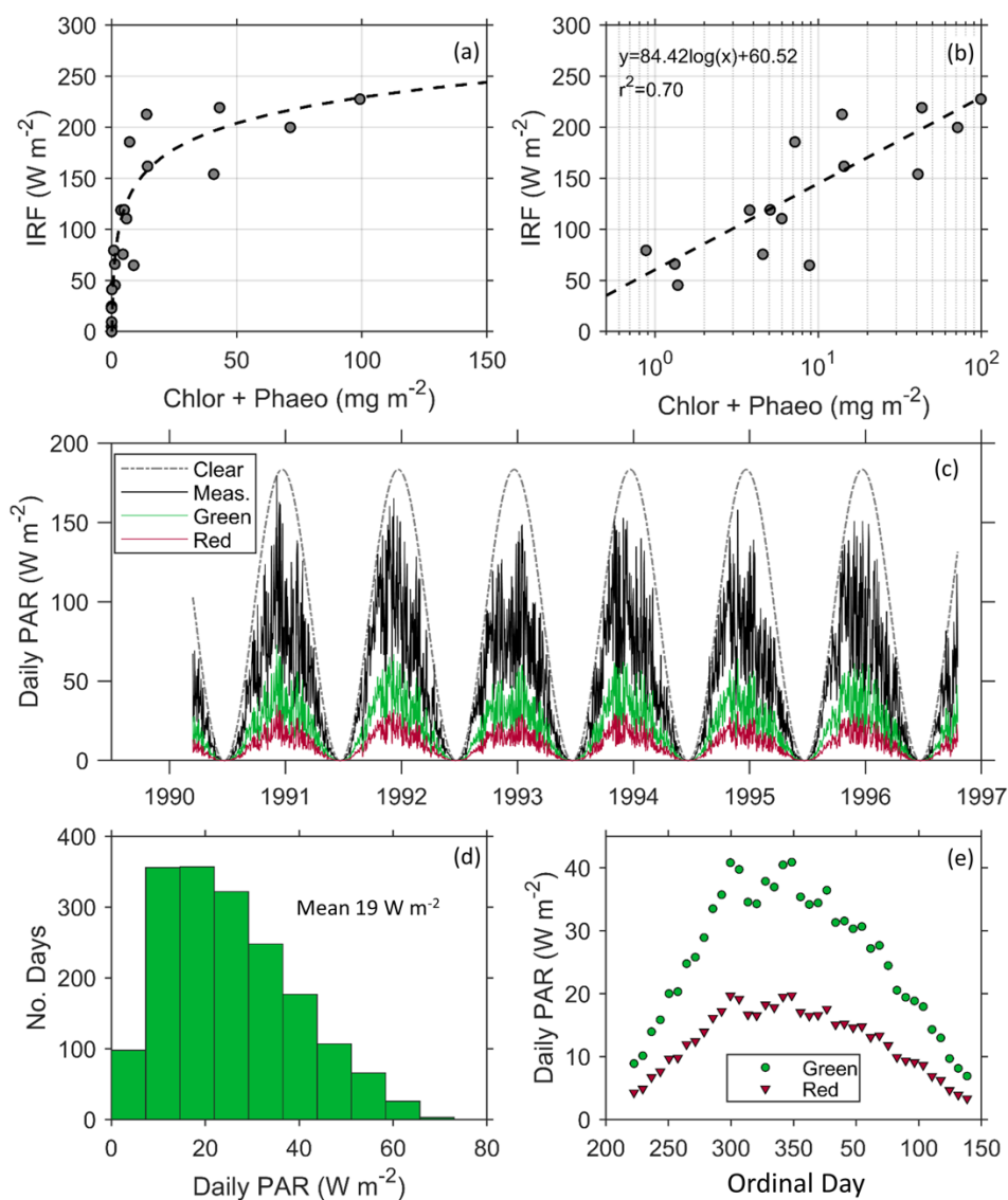
Figure 6. A) Instantaneous radiative forcing (IRF) under clear skies increases with increasing Chlorophyll a and 665 phaeopigment concentrations and B) is modelled using a linear relationship with the logarithmic concentration of pigment. C) Daily PAR measured at Palmer Station (Dierssen et al. 2000) indicates the prevalence of clouds compared to clear sky (dotted line) and provides a daily average radiative forcing (RF) due to red and green algae. D) A histogram showing the daily forcing of green algae follows a slightly skewed pattern with a mean of 19 \text{ W m}^{-2} . E) The daily RF of green and red algae averaged weekly over the course of the growing season at Palmer Station.
