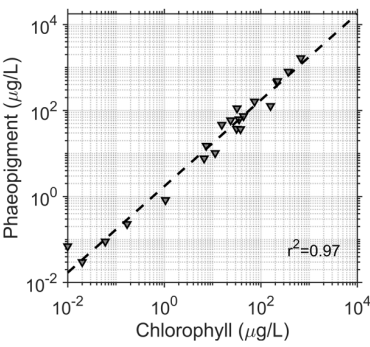
Figure 2: Correlation between Chlorophyll and Phaeopigments for all samples ( R^2=0.97 ) with a slope of 2.34. Concentrations were added together for the subsequent analysis.
