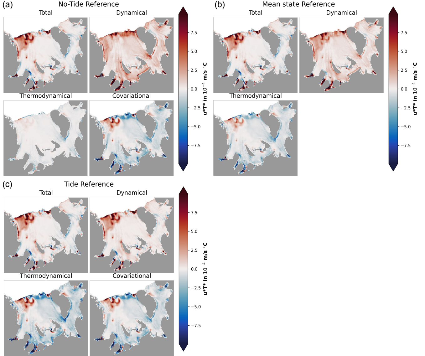
Figure C1. Dynamical-Thermodynamical Decomposition: The impact of the reference state. Contributions of thermodynamical, dynamical and covariational effects to tidal melting when choosing (a) the no-tide experiment, (b) the mean between no-tide and tide case and (c) the tide experiment as reference. The mathematical descriptions for each case are shown in equation C1, C2 and C4, also explaining why the central case has no covariational contribution. For the Tide Reference case the negative of the total, dynamical and thermodynamical contributions have been plotted for better comparison. The contributions are sensitive to the choice of the reference.
