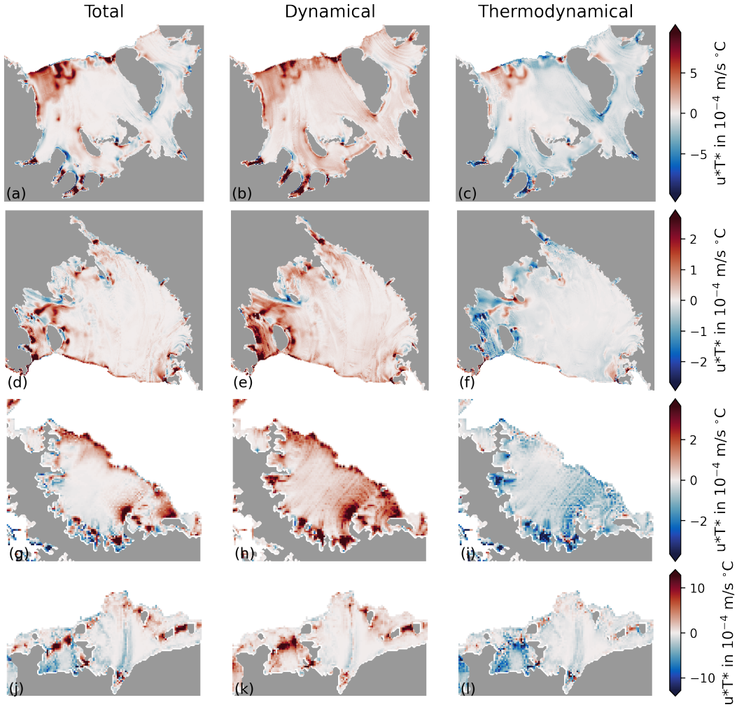
Figure 5. Dynamical-Thermodynamical decomposition of tidal melting under Filchner-Ronne Ice Shelf in cold regimes . Difference in melting, when accounting for (a) all components, (b) only the dynamical component, (c) and only the thermodynamical component and for Filchner-Ronne (a to c), Ross (d to f) only the covariational component, Larsen C (g to i), and Jelbart and Fimbul Ice Shelf (j to l); following Eq. 6).
