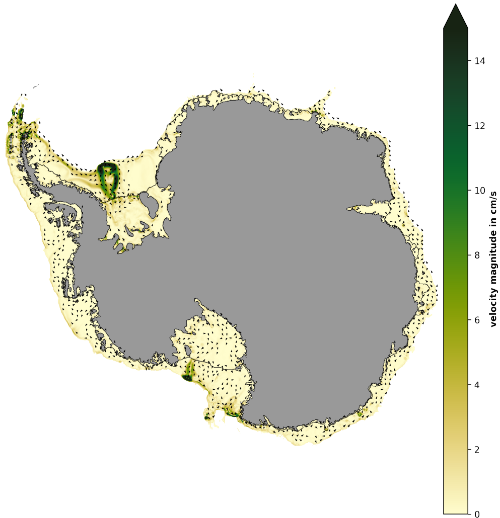
Figure D1. Tidal residual circulation from tide-topography interaction. ?? Annual mean circulation of a tidal simulation without surface forcing, but for the Totten-Moscow University Ice Shelf System thermodynamic ice shelf interaction and stratification.
