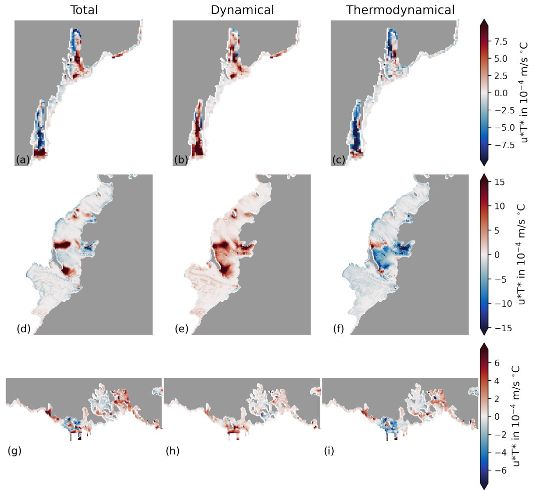
Figure B2. Dynamical-Thermodynamical decomposition of tidal melting under the Amery-Totten-Moscow University Ice Shelf system (a to c), Riiser-Larsen Ice Shelf (d to f) and the ice shelves of the eastern Ross Sea (g to i; see Sec. 2.3).
