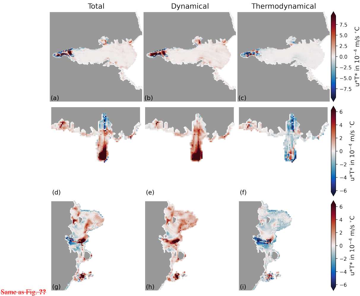
Figure B1. Dynamical-Thermodynamical decomposition of tidal melting under Amery (a to c), but for the Larsen C-Mertz (d to f) and Shackleton Ice Shelf (g to i; see Sec. 2.3).
