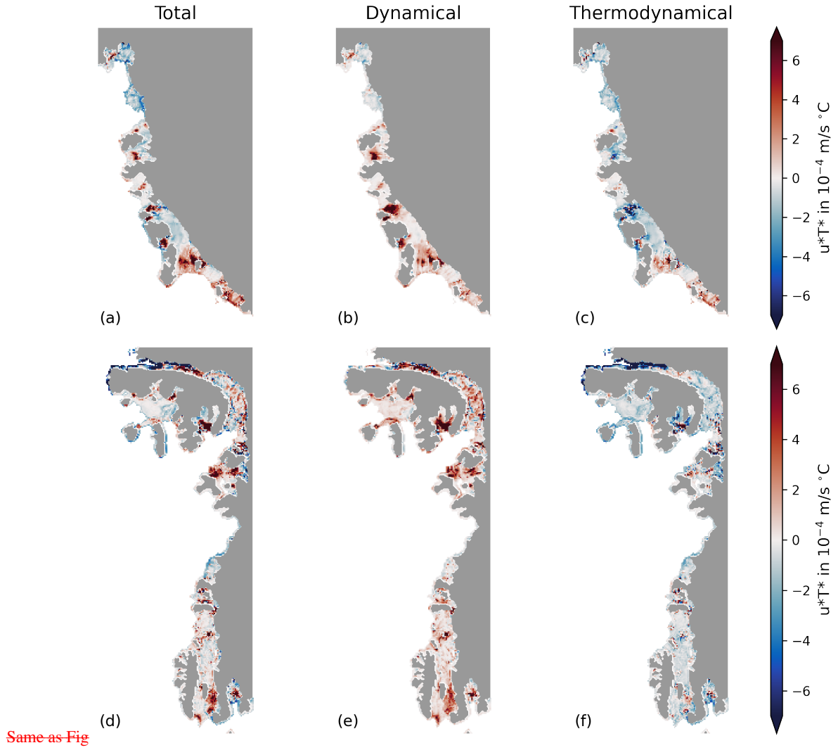
Figure 6. Dynamical-Thermodynamical decomposition of tidal melting in warm regimes. ??Difference in melting, but when accounting for all components, only the dynamical component and only the thermodynamical component for the ice shelves of the Amundsen (a to c) and Bellingshausen Sea (d to f; following Eq. 6).
