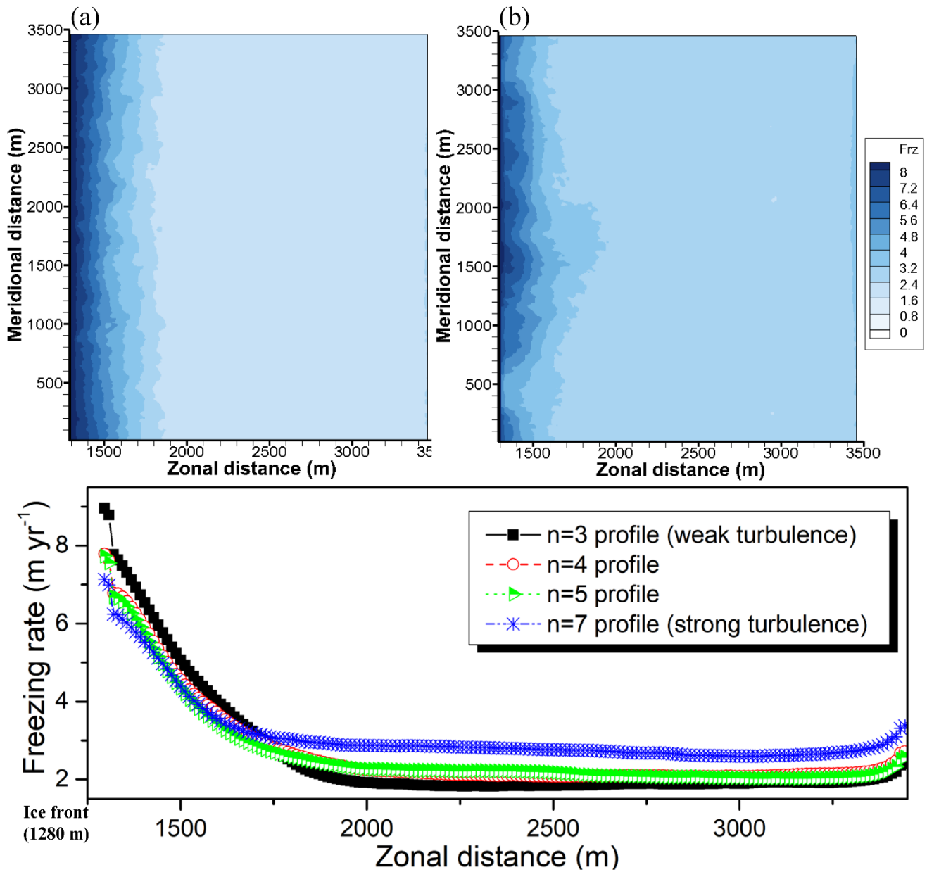
675 Figure 4: XY horizontal distribution of the 3 t^* time-averaged freezing rate (m yr -1 ) at the sea surface. (a) n = 3 , weak turbulence. (b) n = 7 , strong turbulence (c) Zonal-spatial distribution of the freezing rate in the four different turbulence cases. These values are averaged along the meridional direction.
