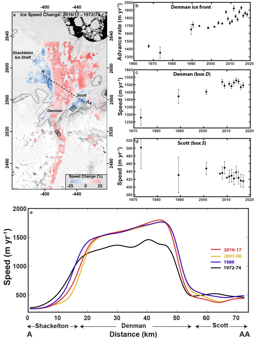
Figure 3: a) Percentage difference in ice speed between 2016-17 and 1972-74 overlain on a Landsat-8 image from November 2017 provided by the U.S. Geological Survey. Red indicates a relative increase in 2016-17 and blue a relative decrease in 2016-17. The grounding line is in grey (Depoorter et al., 2013) b) Time series of the advance rate of the Denman ice-front 1962-2018. c) Time series of mean ice speed from box D, 1972-2017) approximately 10 km behind the Denman grounding line. d) Time series of mean ice speed from box S, on Scott Glacier, 1972-2017. e) Ice speed profiles across the Shackleton-Denman-Scott system from 1972-74, 1989, 2007-08 and 2016-17. Note the lateral migration of the shear margins.
