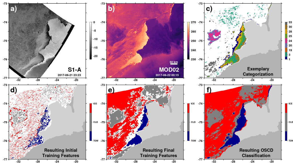
Figure 3. Exemplary generation of labeled training data with reference Sentinel-1 A/B calibrated backscatter image (in dB; a), MOD02 derived ice-surface temperature (in K; b), an exemplary subset of nine clusters out of the 35 total clusters from the used Autoencoder and Fuzzy C-Means Clustering before (c) and after (d) manual categorization and quality control (d; thin-ice/open-water, TOW; clouds, CLD; sea ice, ICE), as well as the final training based on the generalizing NN (e), and the resulting classification based on the final OSCD algorithm (f). Land-ice (dark gray) and ice-shelf (light gray) overlays originate from Rtopo-2 (Schaffer et al., 2016). In (c), clusters 20 and 24 were categorized as 'cloud'; clusters 1, 3, 25, 28, and 30 as 'open-water/thin-ice'; and clusters 19 and 33 as 'sea ice'.
