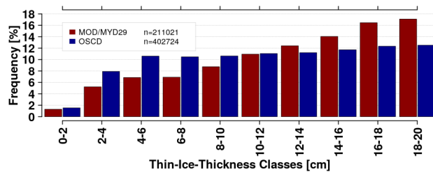
Figure 10. Comparison of binned thin-ice-thickness classes with a bin size of 2 cm based on all available swaths from 1 April to 30 September 2017 between the use of MOD/MYD29 (red) and OSCD (blue) data (b) for the primary BIS polynya (blue dashed outline in Fig. 9).
