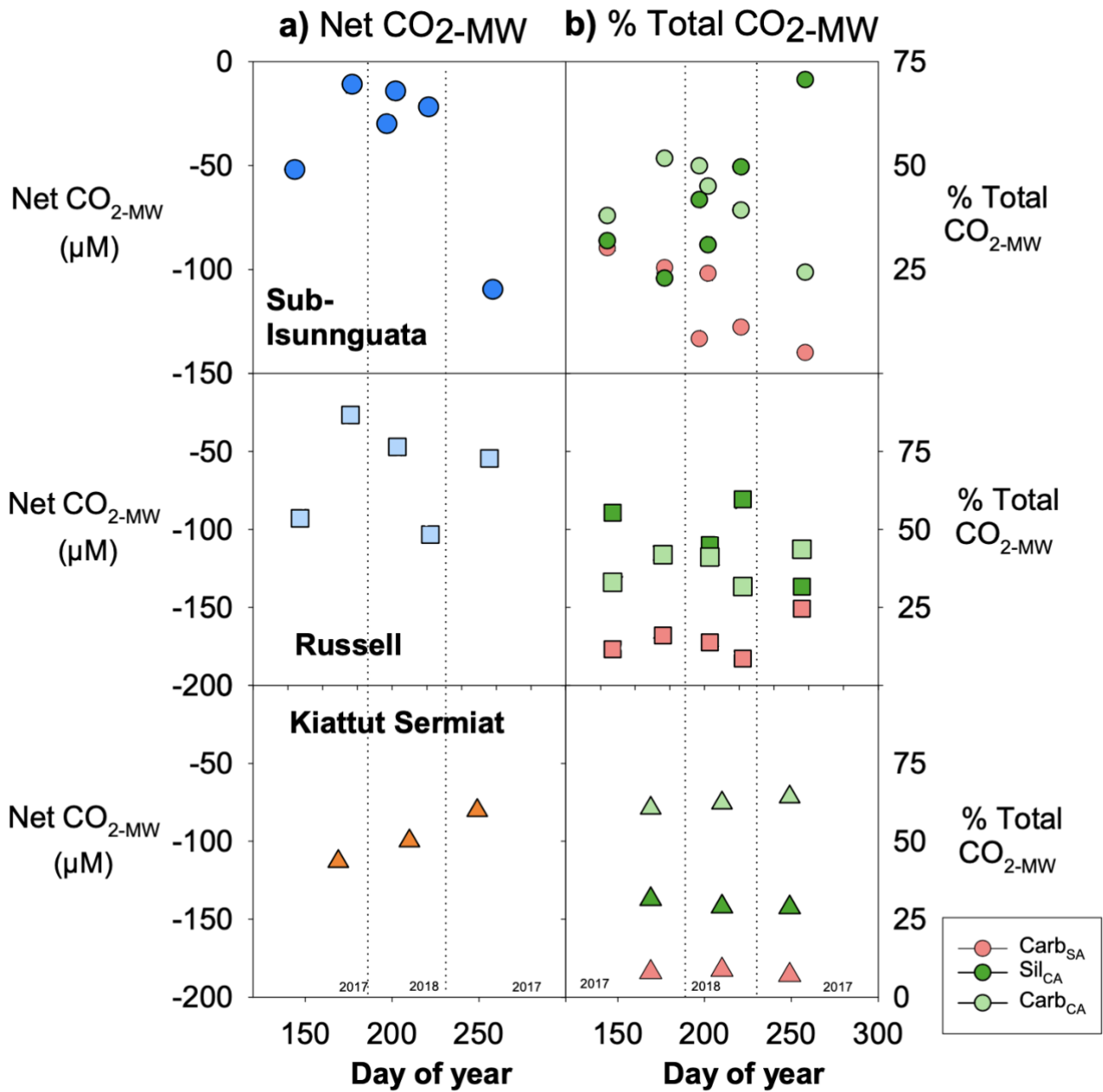
Figure 6. Mineral weathering model results in a) net impact of mineral weathering reactions on CO 2 (Net CO 2-MW ; Eq. 7) for sub-Isunnguata, Russell, and Kiattut Sermiat subglacial discharge sites (where negative values of Net CO 2-MW indicate net sequestration of CO 2 due to mineral weathering), and b) the proportional contribution of each mineral weathering reaction to the total change in CO 2 (% Total CO 2-MW Eq. 9a-9c).
