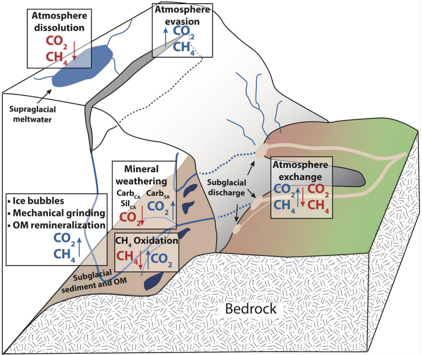
Figure 1: Conceptual diagram of subglacial sources and sinks of \text{CO}_2 and \text{CH}_4 . Arrows indicate the direction of fluxes. Boxes represent processes, and sources of gases to subglacial meltwaters are indicated by blue text while sinks of gases to subglacial meltwater are indicated by red text. Gas bubbles, mechanical grinding, and OM remineralization are grouped because all are \text{CO}_2 and \text{CH}_4 sources.
