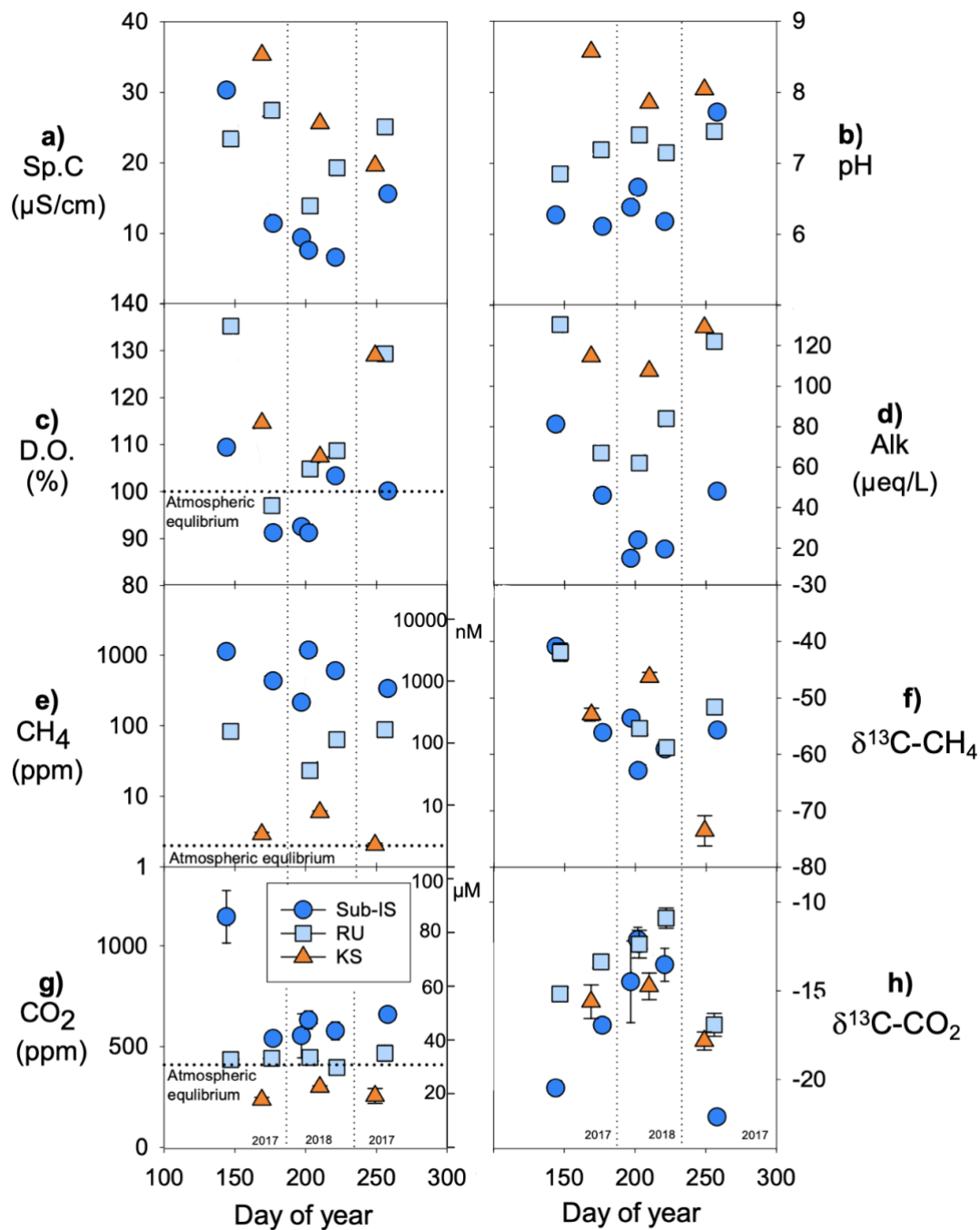
Figure 3. Chemical parameters at sub-Isunnguata (sub-IS), Russell (RU) and Kiattut Sermiat (KS) subglacial water sampling sites versus day of year for a) specific conductivity (Sp.C), b) pH, c) dissolved oxygen (D.O.) percent saturation, d) alkalinity (Alk), e) measured \text{CH}_4 concentrations (left y-axis in ppm and right y-axis in nM), f) \delta^{13}\text{C}-\text{CH}_4 values, g) measured \text{CO}_2 concentrations (left y-axis in ppm and right y-axis in \mu\text{M} ), and h) \delta^{13}\text{C}-\text{CO}_2 values. Atmospheric equilibrium concentrations are indicated by dashed lines and taken as 1.9 ppm for \text{CH}_4 and 410 ppm for \text{CO}_2 . Error bars on \text{CH}_4 and \text{CO}_2 concentrations and stable isotopic compositions represents the standard deviation of replicates and are smaller than symbols for some data points.
