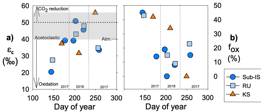
1270 Figure 4. CH 4 dynamics over the course of the 2017 and 2018 melt seasons including a) the carbon fractionation factor ( \epsilon_c ) between 1275 dissolved CO 2 and CH 4 and b) the fraction of CH 4 oxidized ( f_{ox} ) for sub -Isunnguata (IS), Russell (RU) and Kiattut Sermiat (KS) samples. Fields of \epsilon_c representing methanogenesis and oxidation values are based on Whiticar (1999). Values of \epsilon_c between approximately 40 and 55 (gray shaded region in panel a) are produced for methanogenesis via acetate fermentation, while CO 2 reduction produces values between approximately 50 and 90. Lower values result from a predominant isotopic signature of CH 4 oxidation. Atmospheric input without additional alteration of CO 2 or CH 4 isotopic systematics results in a \epsilon_c value of approximately 40.
