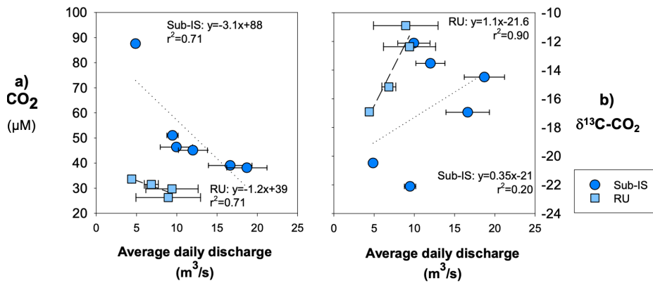
310 Figure 8. Relationships between average daily discharge a) CO 2 concentrations, and b) δ 13 C-CO 2 . Regressions are shown by dotted lines for sub-Isunnguata and dashed lines for Russell samples. Horizontal error bars represent the standard deviation of average daily discharge for days samples were collected and are smaller than symbols for some data points.
