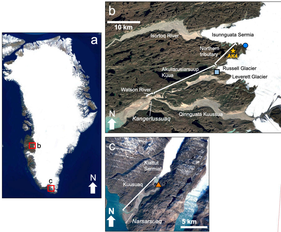
245 Figure 2. Google Earth satellite images of study locations in a) Greenland including b) locations near the town of Kangerlussuaq, including the sub-Isunnguata water sampling location (dark blue circle) and Russell water sampling location (light blue square). The gold star represents the location of AK4, where proglacial river discharge records were collected. (c) Location of Kiattut Sermiat site (orange triangle) near the town of Narsarsuaq in southern Greenland, where water samples were collected.
