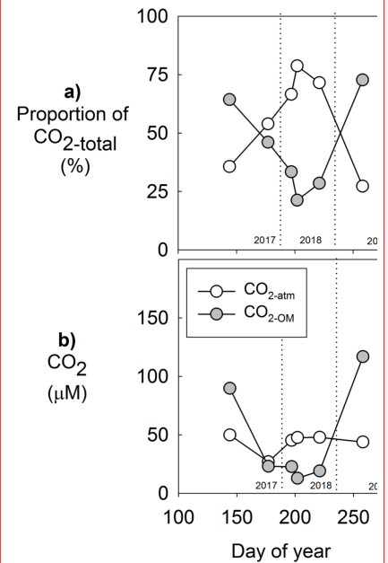
Figure 9. Estimates of contributions of atmospheric \text{CO}_2 ( \text{CO}_2\text{-atm} ) compared to that derived from remineralized OM ( \text{CO}_2\text{-OM} ) for Isunnguata subglacial discharge site including a) relative contributions according to the day of the year, b) absolute ... [8]
