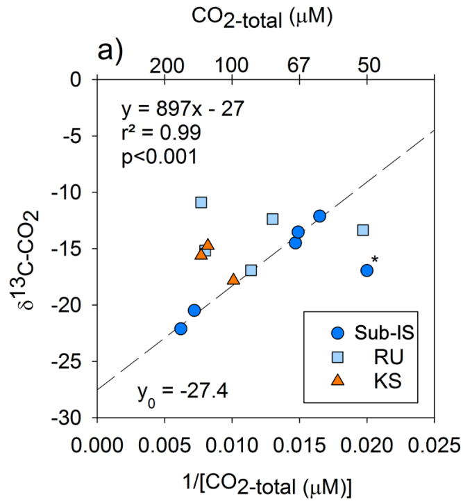
Figure 9. Keeling plot indicating correlations between the magnitude of \text{CO}_2\text{-total} and \delta^{13}\text{C-CO}_2 and for sub-Isunnguata (sub-IS), Russell (RU) and Kiattut Sermiat (KS) samples. Asterisk denotes the outlier not included in the regression between \text{CO}_2\text{-total} and \delta^{13}\text{C-CO}_2 for sub-Isunnguata samples. The plotted regression line was constructed using the sub-IS samples only.
