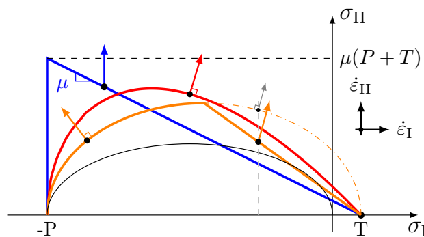
Figure 1: New Fig. 8. Caption: Alternative yield curves and flow rules: The Mohr-Coulomb yield curve with shear, non-normal, flow rule (blue Ip et al., 1991), the modified Coulombic yield curve with normal (elliptic part) and non-normal (linear part) flow rule (orange, Hibler and Schulson, 2000), and the teardrop yield curve with a normal flow rule (red, Zhang and Rothrock, 2005). The elliptical yield curve with e_F = 2.0 is shown for reference (black thin line). P is the compressive ice strength, and T the tensile ice strength.
