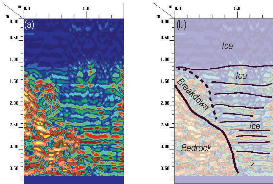
785 Figure 6. Results of an 8-m long Ground Penetrating Radar (GPR) survey across the Icicle Room, presenting uninterpreted (a) and interpreted (b) data. From the surface to a depth of ~1 m the ice is only faintly stratified, whereas below that depth the ice contains increasingly prominent radar reflectors. The steeply sloping bedrock surface is defined on the left side of the transect, mantled in places by breakdown. The maximum thickness of ice here is unclear, but it may be in excess of the 3.5 m penetrated by the 400 MHz GPR system.
