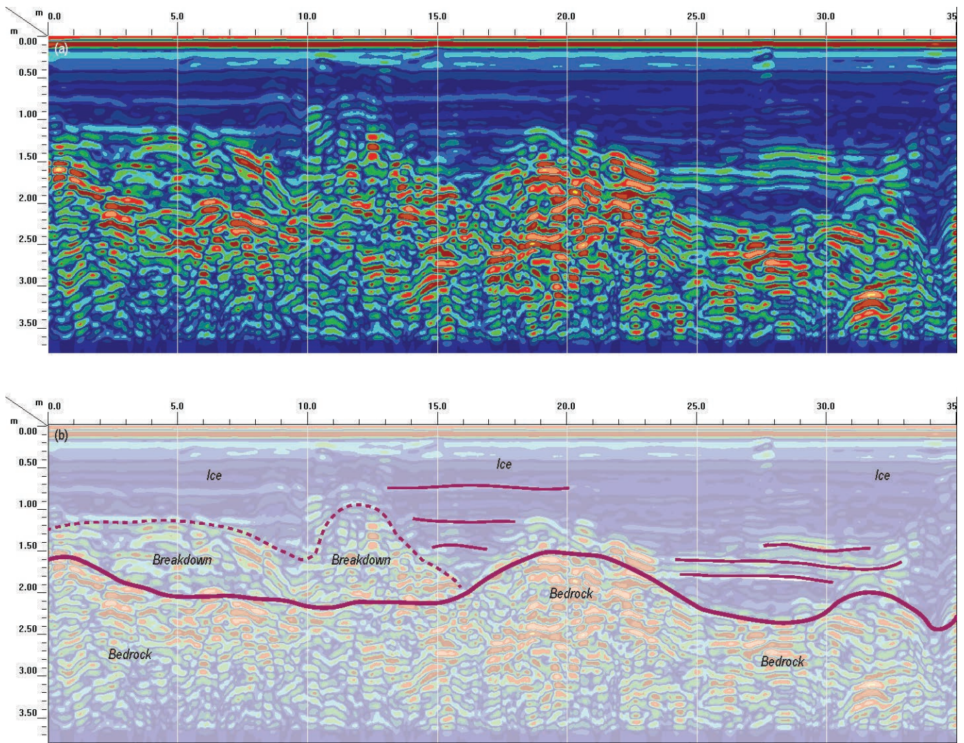
Figure 5. Results of a Ground Penetrating Radar (GPR) survey along the Frozen Freeway. (a) Uninterpreted GPR data for half of the full survey length, with the back of the cave on the right. Vertical white lines mark measured points every 5 m used for scaling the GPR survey. (b) Interpretation of the GPR survey shown in (a). The bedrock surface is represented by an irregular, but laterally continuous contact. More isolated and discontinuous zones of high amplitude reflectors above this contactor interpreted as piles of breakdown. Ice beneath the Skating Rink, between 20 and 35 m along the transect, reaches a maximum thickness of nearly 2.5 m. Ice along the Frozen Freeway, between 0 and 20 m, has a maximum thickness of ~2 m. Horizontal lines within the ice are interpreted as stratigraphic layers.
