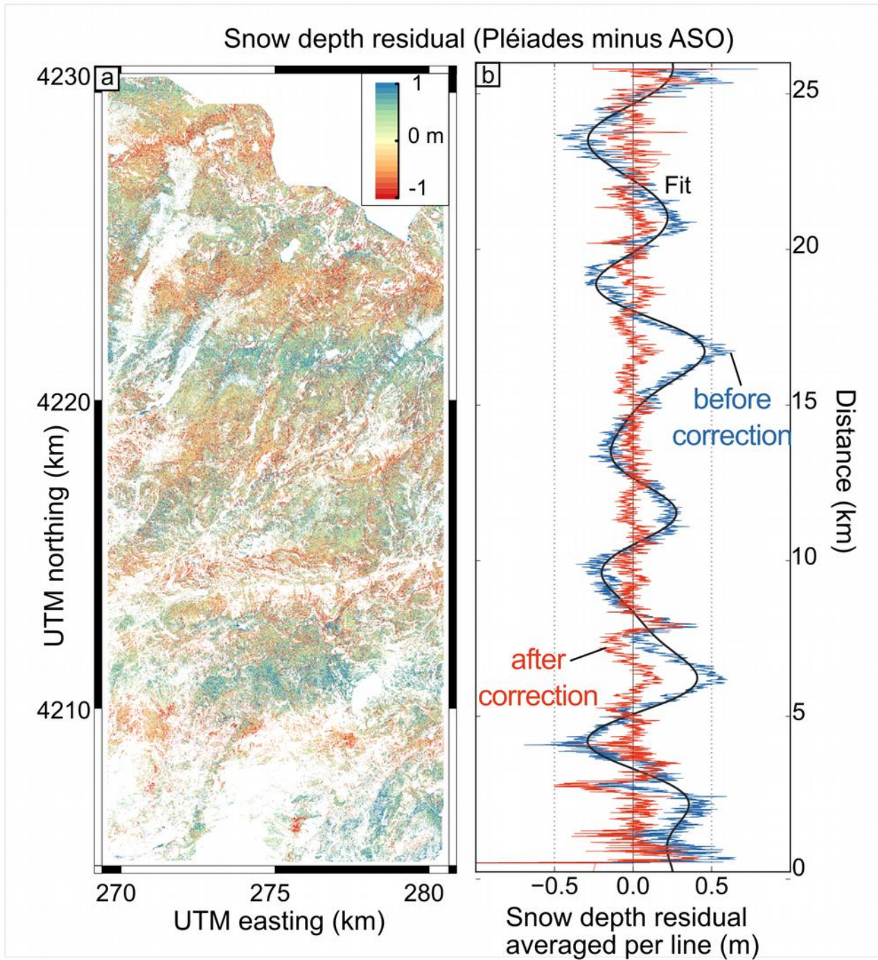
625 Figure 8. Residual snow depth (Pléiades minus ASO) over the complete study area (a) and average per line (b). In b., the HS residual before correction (blue) is corrected for the low frequency undulation (black) to obtain a corrected signal (red).
