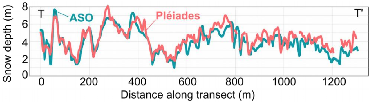
Figure 5. Transect T-T' of snow depth visible on Figure 4. e. from Pléiades data (pink) and ASO (blue). More transects are available in supplement (Figure S3 and S4).
