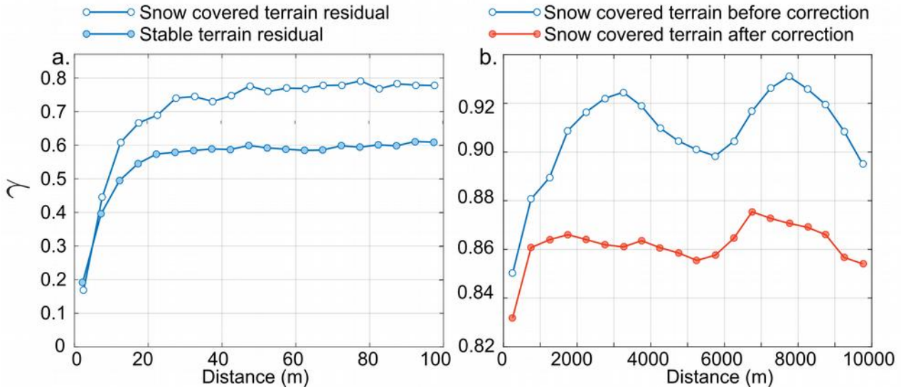
Figure 9. (a) Semi-variogram or spatial autocorrelation ( \gamma ) against lag distance of the HS residuals (empty circles) and Pléiades elevation difference over stable terrain (filled circle). (b) Semi-variogram of the HS residuals for large distances before (blue line) and after correcting the undulation pattern (red line), illustrating the reduction in spatial variance at greater lag distances due to this correction (Sect. 6.5).
