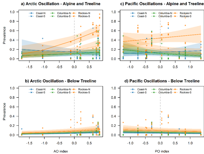
475 Figure 8: Calculated prevalence for Deep persistent slab avalanche problems in relation to AO (left column) and Pacific-centered oscillations (right column) for the alpine/treeline (top row) and below treeline (bottom row) over the range of observed index values. Lines indicate the mean estimates and shaded areas represent that 95% confidence intervals. Individual points represent observed prevalence values.
