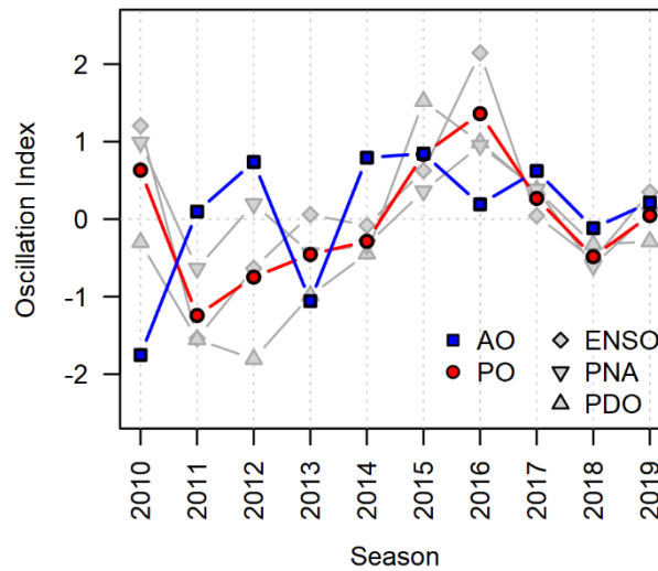
255 Figure 3: Winter season (Nov. – Apr.) average climate indices during the study period (ENSO: El Nino-Southern Oscillation; PNA: Pacific North America Teleconnection Pattern; PDO: Pacific Decadal Oscillation; AO: Arctic Oscillation, PO: Averaged Pacific-centered oscillations).
