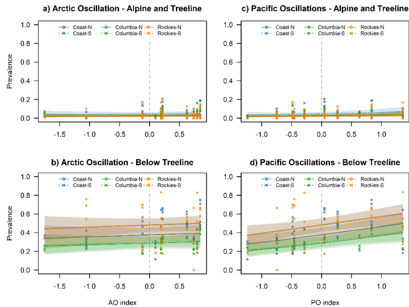
470 Figure 7: Calculated prevalence for No avalanche problems in relation to AO (left column) and Pacific-centered oscillations (right column) for the alpine/treeline (top row) and below treeline (bottom row) over the range of observed index values. Lines indicate the mean estimates and shaded areas represent that 95% confidence intervals. Individual points represent observed prevalence values.
