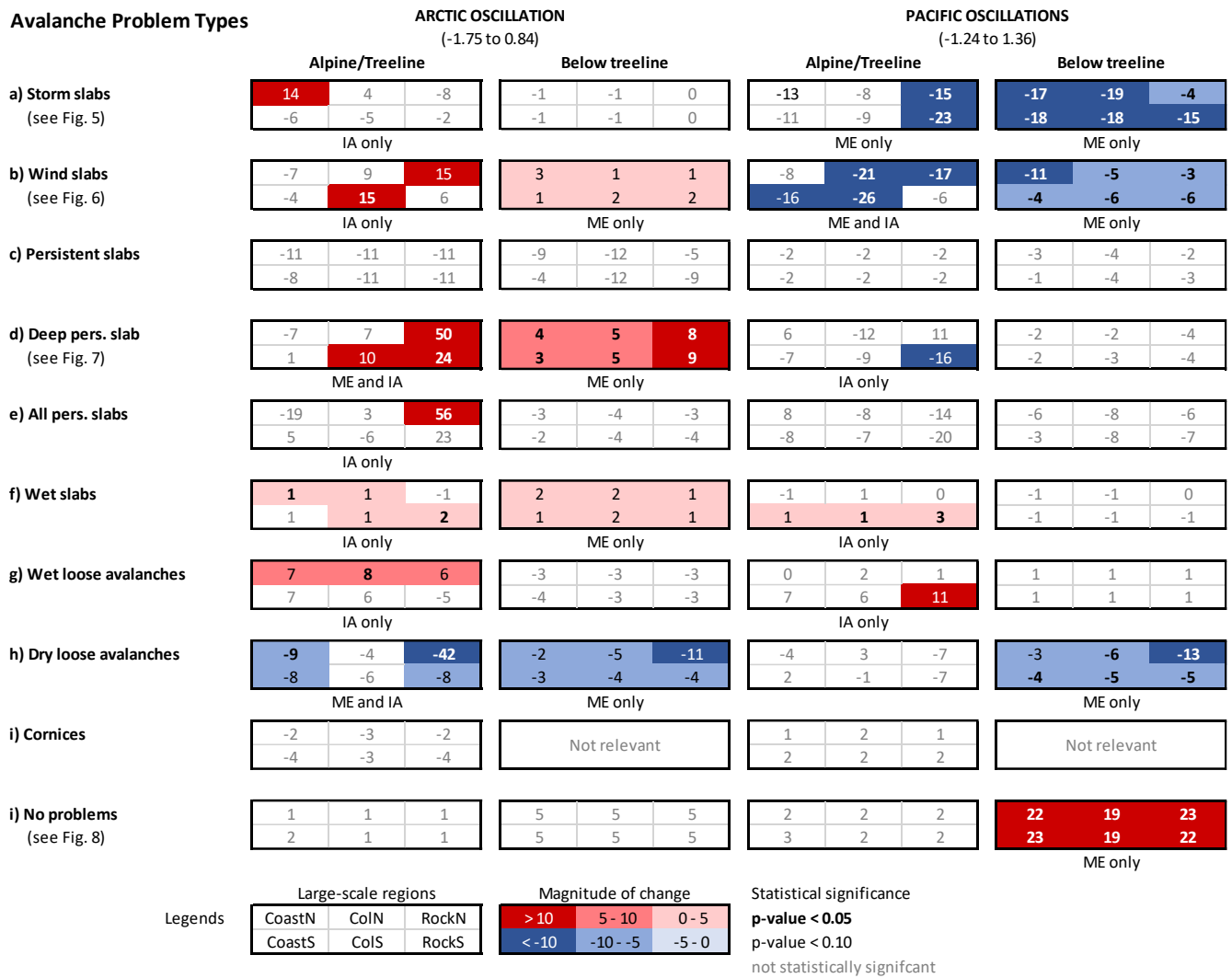
Figure 4: Overview of the effect of the examined atmospheric oscillations on the prevalence values of avalanche problem types expressed as change in percentage points over the range of the observed oscillation indices (i.e., difference in marginal mean estimates). For each avalanche problem type and elevation band (alpine/treeline and below treeline) the six percentage point values are arranged to roughly represent their geographic arrangement. Font weight and color of the percentage point labels describe the statistical significance of the difference: bold and black/white: p < 0.05 ; black/white only: 0.05 \leq p < 0.10 ; grey: not statistically significant. The shading of the cell indicates the magnitude of any significant percentage point differences: dark blue: < -10 pp; medium blue: -10 to -5 pp; faint blue: -5 to 0 pp; faint red: 0 to 5 pp; medium red: 5 to 10 pp; dark red: > 10 pp. The labels underneath the boxes indicate whether the model includes significant the main (ME) and/or interaction effects (IA).
