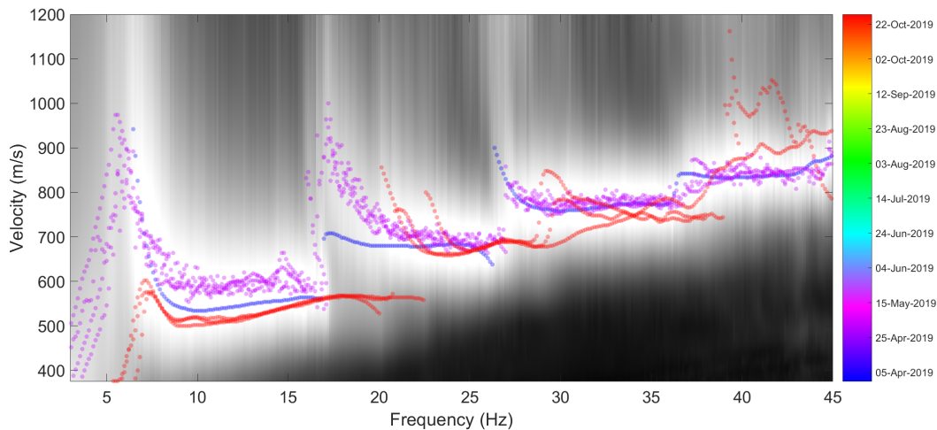
Fig. 1. Dispersion trends for a spatially clustered subset of microseismic events. We observe significant variation between spring and autumn events.
