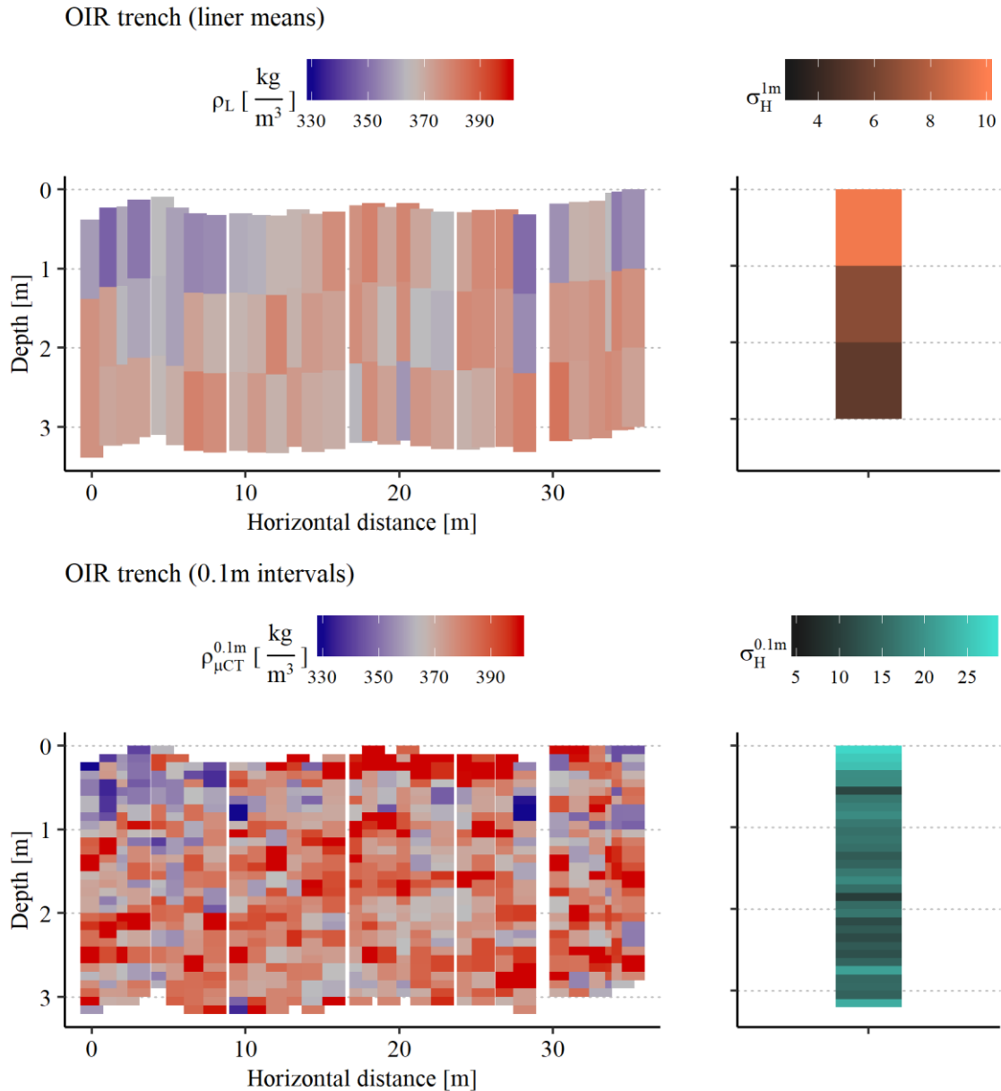
Figure 5: Density of the OIR trench from 30 profiles in vertical 1 m (liner density, top) and 0.1 m sampling intervals ( \mu\text{CT} density, bottom) in a color-coded plot. For the profiles in 0.1 m intervals, we used a common depth scale for the whole trench starting at the top of the profile with the highest surface elevation (profile 30), all other liners start at the measured relative height. We then calculated the density of each 0.1 m interval according to the common depth scale. \rho_L and \rho_{\mu\text{CT}}^{0.1m} , respectively, are given in a blue (low density) to red (high density) color code. On the right of each panel \sigma_H of the respective depth interval is shown.
