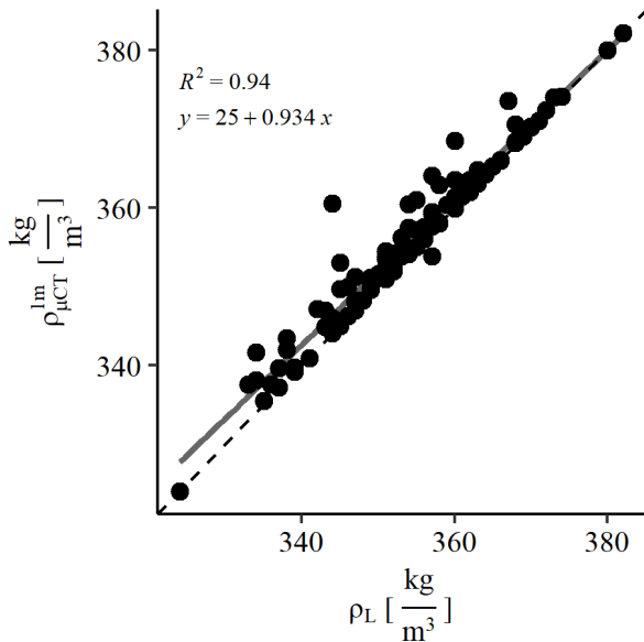
Figure 4: Comparison of liner density ( \rho_L ) with \mu CT density ( \rho_{\mu CT}^{1m} ) calculated from the 114 liners along the traverse. Values of both measurements are in good agreement with an R^2 of 0.94. The linear fit is given with a grey solid line, the dashed black line represents x=y .
