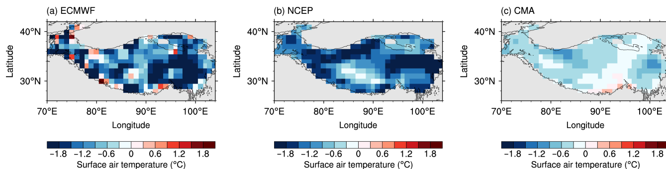
645 Figure 9. Differences in the multiyear wintertime mean surface air temperature over the Tibetan Plateau (unit: °C) between forecasts with a lead of 4 weeks and forecasts with a lead of 1 week in (a) ECMWF, (b)NCEP and (c) CMA. The map of Tibetan Plateau was created by using Global Relief Model data of ETOPO1, topographic data free to the public (doi:10.7289/V5C8276M).
