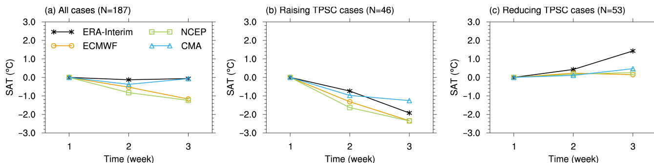
655 Figure 10. Composites of surface air temperature over the Tibetan Plateau (unit: °C) for (a) all cases, (b) increasing TPSC cases, and (c) decreasing TPSC cases. Black lines, orange lines, green lines, blue lines and black lines represent composites in observation, ECMWF, NCEP, and CMA, respectively; see legend in (a). The x-axis represents the number of weeks in the cases for the composites, which are also forecast lead times (unit: week). The “N” in the title of each plot indicates the number of cases for the composite.
