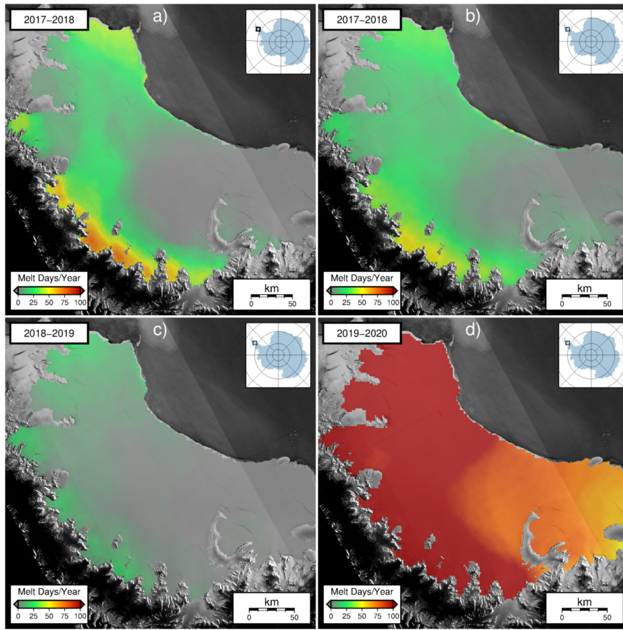
Figure 2. Number of melt days in the three most recent melt seasons a) 2017/2018 based on SIR ASCAT data, calculated using b) 2017/2018 based on Level 1 ASCAT data, c) 2018/2019 based on Level 1 ASCAT data, and d) 2019/2020 based on Level 1 ASCAT data. The background image is Copernicus Sentinel-1 2019 mean backscatter.
