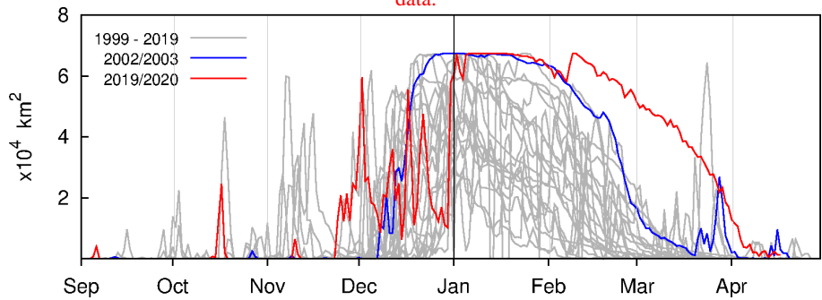
Melt index time series based on brightness temperatures from SMMR and SSMI, SIR QuikSCAT and ASCAT data, and Level 1 ASCAT data.
