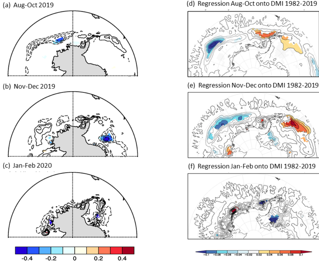
Figure A4. Left panels: Anomaly Anomalies in sea ice concentration relative to the 1981 to 1982–2019 climatological mean for a) August, September and October 2019, b) November and December 2019, c) January and February 2020. Shading is as in Fig. A2. Right panels: Linear regression of sea ice concentration anomaly onto the Dipole Mode Index (DMI) for the equivalent period based on data from 1981 1982 to 2019. Shading indicates regression is significant at p < 0.10 . The regression coefficients are scaled by 1 standard deviation of the DMI so that the maps represent the sea-ice sea ice -anomaly that would be accounted for by 1 standard deviation in DMI for d) August to October, e) November to December, f) January to February. The regressions were computed using the Royal Netherlands Meteorological Institute (KNMI) Climate Explorer (see climexp.knmi.nl , Oldenborgh and Burgers, 2005).
