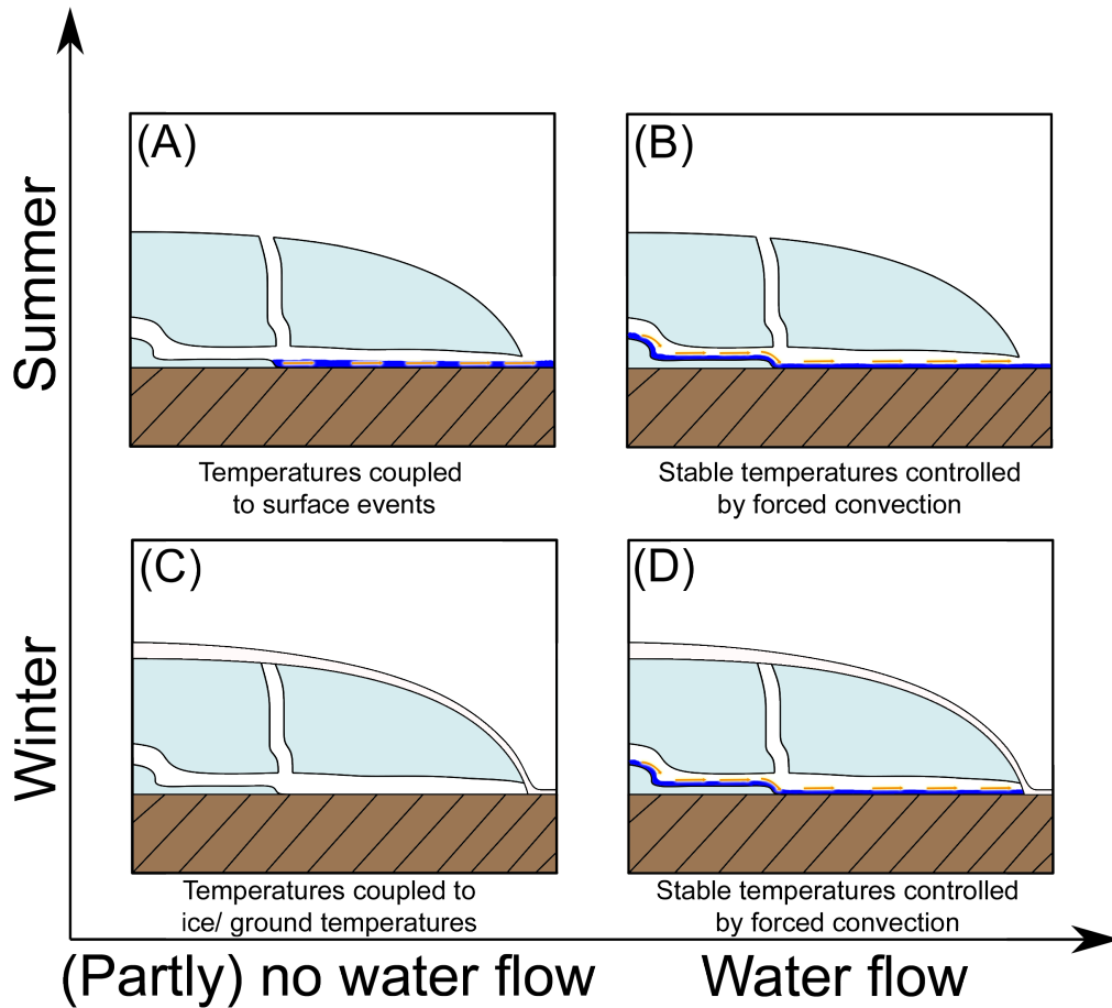
Figure 11. Proposed thermal control phases of subglacial drainage systems. The y-axis shows the difference between summer and wintertime, with orange arrows indicating forced convection. (A) Sections of subglacial temperatures being controlled by surrounding drainage systems under thin ice and sediment can exhibit no water flow during parts of summer (left part of the channel indicated in wintertime and the schematic). The temperatures in these water free sections will be more fluctuating, thereby being coupled to surface weather during summertime events. (B) Presence of running liquid water causes in the whole subglacial drainage system leads to stable temperatures due to in the whole system, which are controlled by the forced convection both caused by the water. (C) Temperatures in summer winter without the presence of additional running water will be less stable again, mainly dictated by the temperatures of surrounding ice/ ground temperatures and natural convection. (D) Running water in winter. Yellow arrows mark air circulation via will again cause forced convection, leading to stable temperatures.
