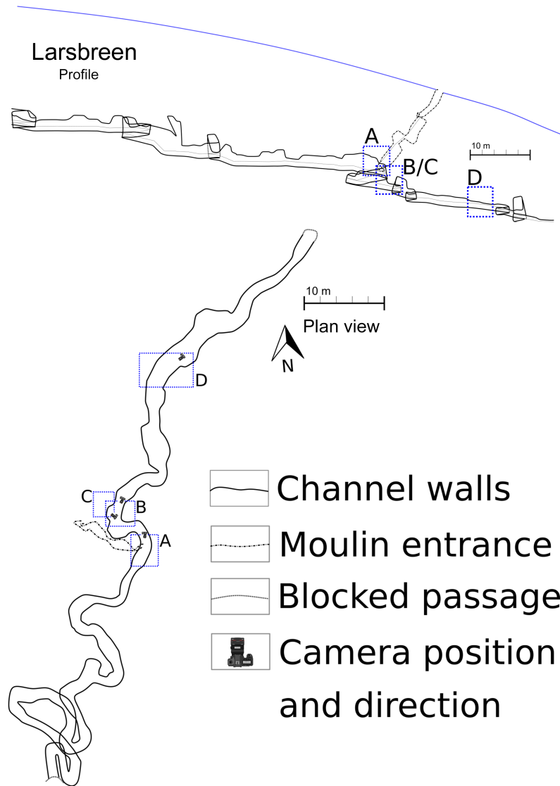
Figure 2. Plan view drainage system map of Larsbreen with picture locations ( center lower sketch ) and vertical cross-section/extended profile (upper sketch) with approximate glacier surface and photos . The drainage system could be entered by rappelling down a moulin/ channel, leading into the subglacial channel at (A). Channel looking upstream, picture taken from sensor location (B) locations. Location of the sensor borehole at the side of the channel marked (C) figure 4. Note that the logger box visible on the picture was later on moved higher up towards the ceiling of the drainage system. Low continuing passage towards the glacier front at (D). Dates of pictures: 7.11.2015 (A), 02.12.2015 (D), 05.03.2016 (B, C).
