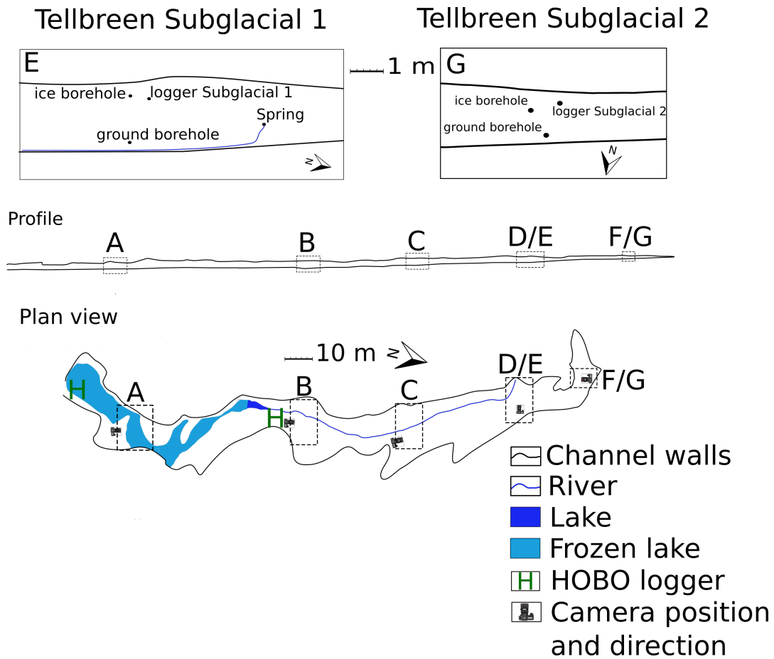
Figure 3. Drainage system map of the Tellbreen subglacial drainage system with plan view and picture locations (lower sketch) and vertical cross-section/extended profile (middle sketch). The channel entrance lies at the south-west, leading into a frozen lake area (A) . One Hobo logger (H) was installed next to the entrance . A small stream is running through a Nye-Channel, filling up the lake throughout winter (B) . Nye-channel further into the subglacial drainage system with stream running on the left side and a person for scale in the picture centre, at the location of the spring (C) . Logger setup next to the spring (D) and at the channel end (E) . All pictures taken on 14.03.2019 can be found in figure 4 .
