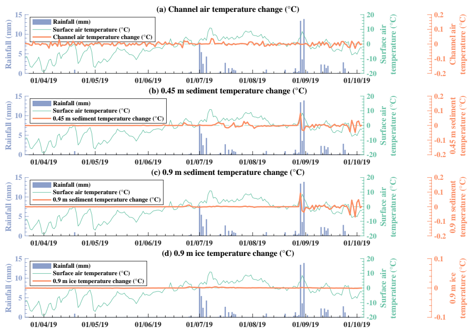
Fig. 2. Change of daily temperatures at logger 'Subglacial 2'.
