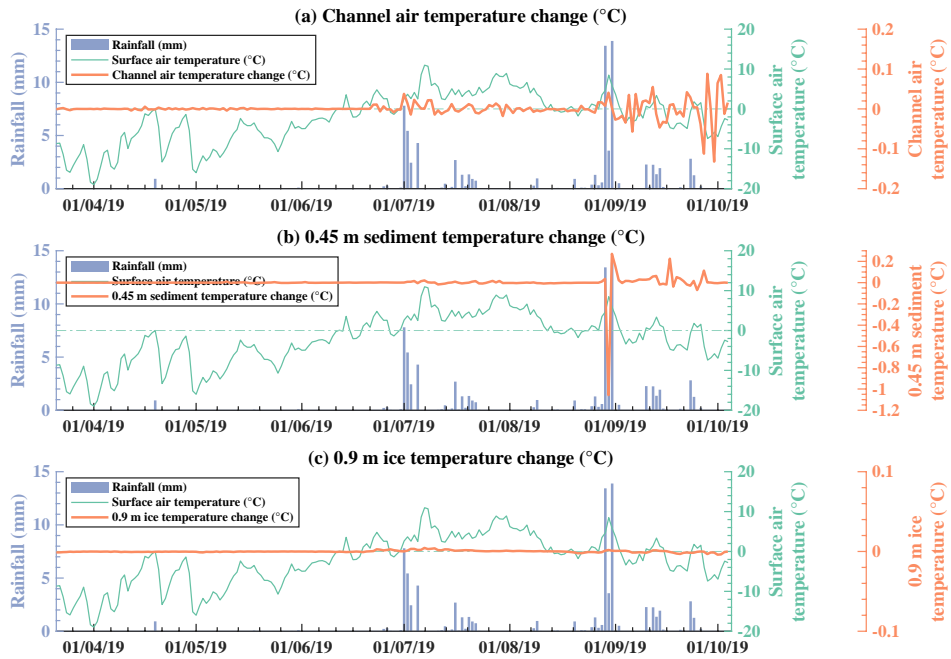
Fig. 1. Change of daily temperatures at logger 'Subglacial 1'.
