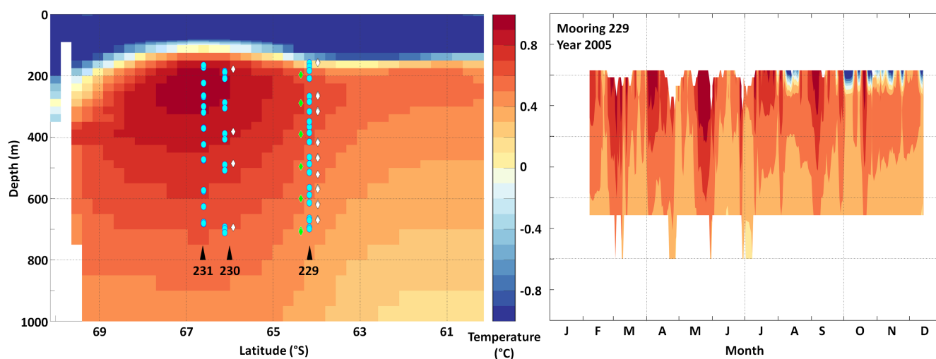
Figure 7. Left: Climatological temperature along the Prime Meridian, from Locarnini et al. (2018), showing the comparatively warm Circumpolar Deep Water in red. For each mooring line (229, 230, and 231), the symbols indicate the depth of the mooring temperature sensors during deployments that coincided with polynya events: white diamonds for 1999 and 2000; cyan circles for 2004 and 2005; and green diamonds for 2016. The latitude shift between deployments of the same mooring is for readability only. Salinity section available as supplementary figure B3. Right: on the same vertical axis (depth from 0 to 1000 m), time series of daily median temperature as recorded by mooring 229 in 2005.
