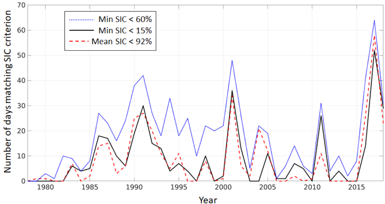
Figure 2. For each year of the sea ice time series (1978-2018), number of days between 1st July and 31st October with a polynya according to the three most common criteria in the literature: black, minimum sea ice concentration (SIC) lower than 15% (e.g. Gloersen et al., 1992); blue, minimum sea ice concentration lower than 60% (Campbell et al., 2019); red, average sea ice concentration over the (fixed) polynya-prone region lower than 92% (after Gordon et al., 2007).
