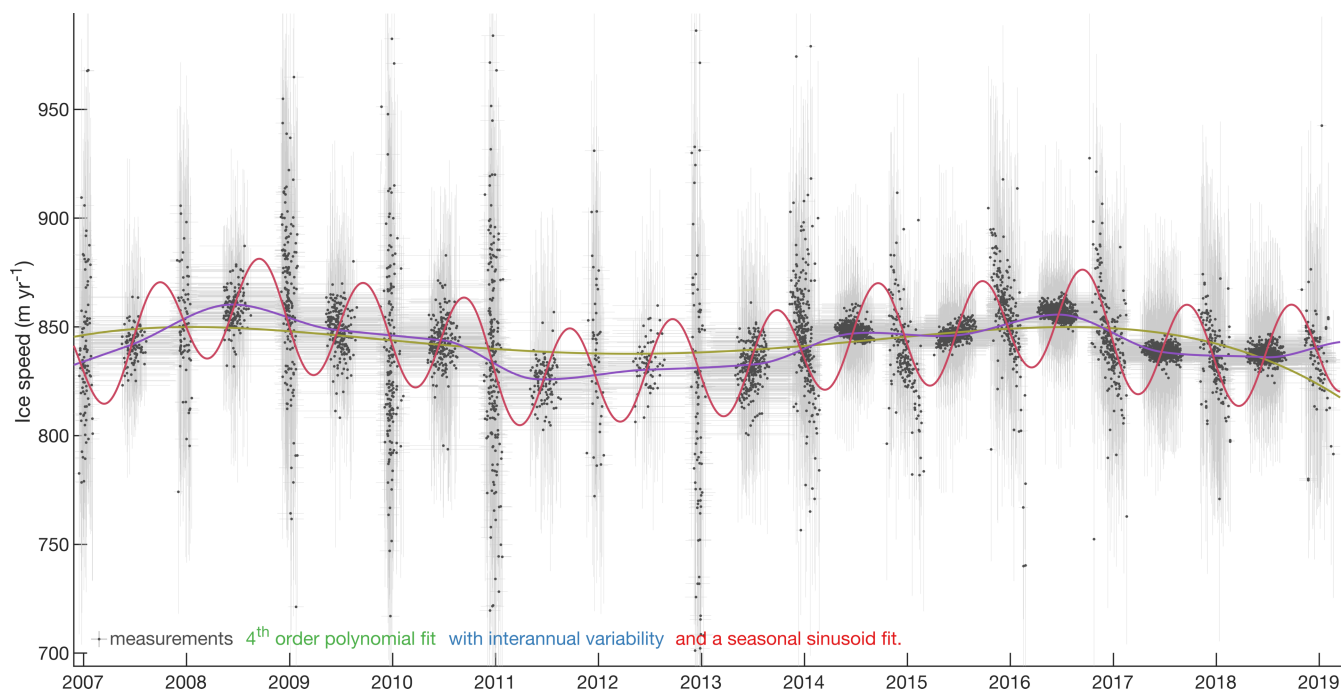
Figure 4. Velocity time series for an ITS_LIVE pixel. These 14,208 measurements taken near the grounding line of Byrd Glacier typify ITS_LIVE image pair data, with short- \Delta t measurements providing direct, but noisy observations of velocity variability throughout each summer, while much lower-noise winter estimates can only give insight into the total displacement that occurs during the dark, winter months. Light gray horizontal bars connect the acquisition times of each image pair and vertical bars show \pm 1\sigma_v uncertainty. Center dates t_m are shown as dark gray dots for visual clarity.
