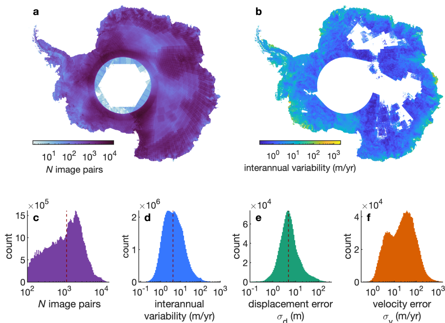
Figure 3. ITS_LIVE velocity data statistics. Maps of a : the number of image pairs that contribute to each 240 \times 240 m pixel in the ITS_LIVE summary velocity mosaic and b : the standard deviation of annual velocity mosaics from 2013 to 2018. Histograms in panels c and d show only the values from a and b that correspond to grid cells with at least 100 contributing image pairs and whose mean velocity is at least 15 \text{ m yr}^{-1} . Displacement errors \sigma_d shown in panel e result from satellite image georegistration error, and when divided by values of \Delta t corresponding to each image pair results in the velocity errors \sigma_v shown in panel f . Because displacement errors are distributed symmetrically, the bimodal distribution of velocity errors roughly correspond to the two peaks of \Delta t values over which velocity is measured (shown in Fig. 2). Vertical lines in panels c–e indicate median values of 1153 image pairs per grid cell, 4.2 \text{ m yr}^{-1} interannual variability, and 4.9 m displacement error.
