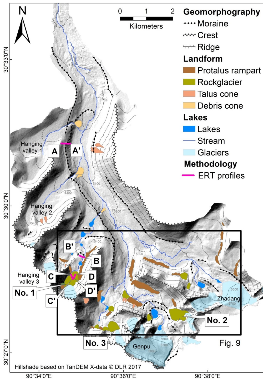
Figure 6: Geomorphological map of the Qugaie basin. The locations of the ERT profiles are shown with purple lines. Periglacial landforms are greenish (rockglaciers and protalus ramparts). The black rectangle represents the boundary of the map shown in Figure 9.
