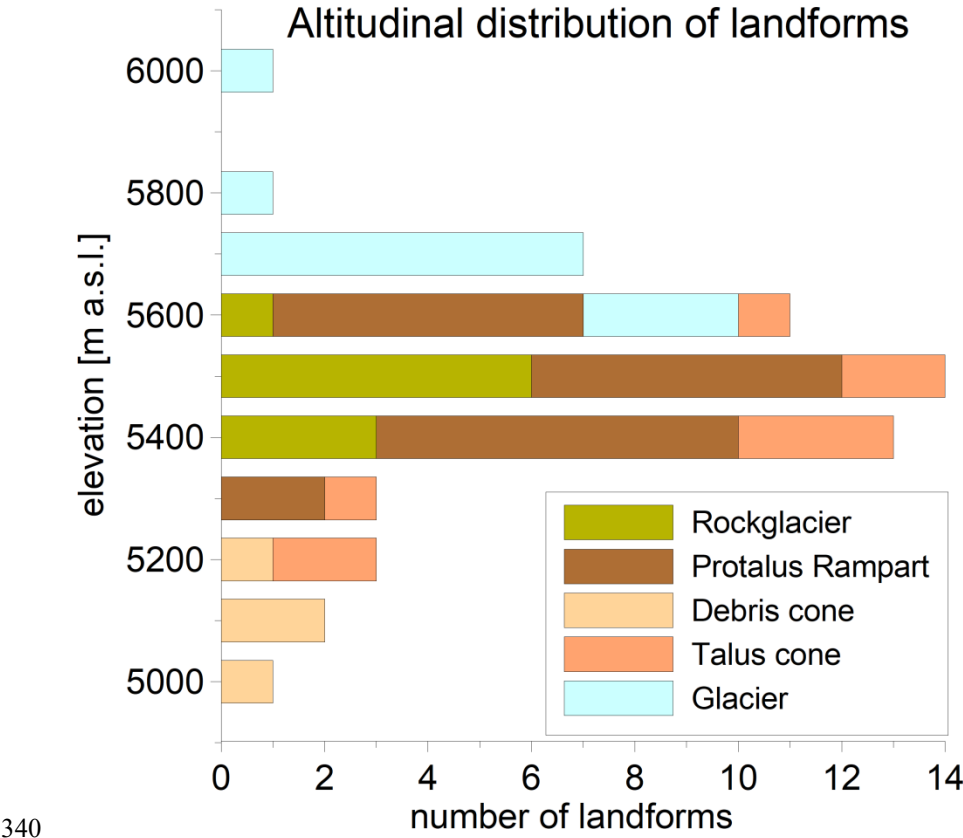
340 Figure 7: Altitudinal (mean) landform distribution of the Qugaqie basin derived from the landform inventory.
