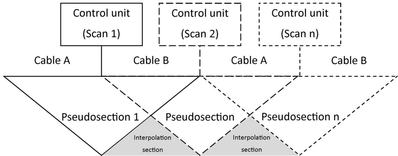
255 Figure 5: Measurement setup for the Roll-along procedure (adapted from N El Sayed et al., 2018).
