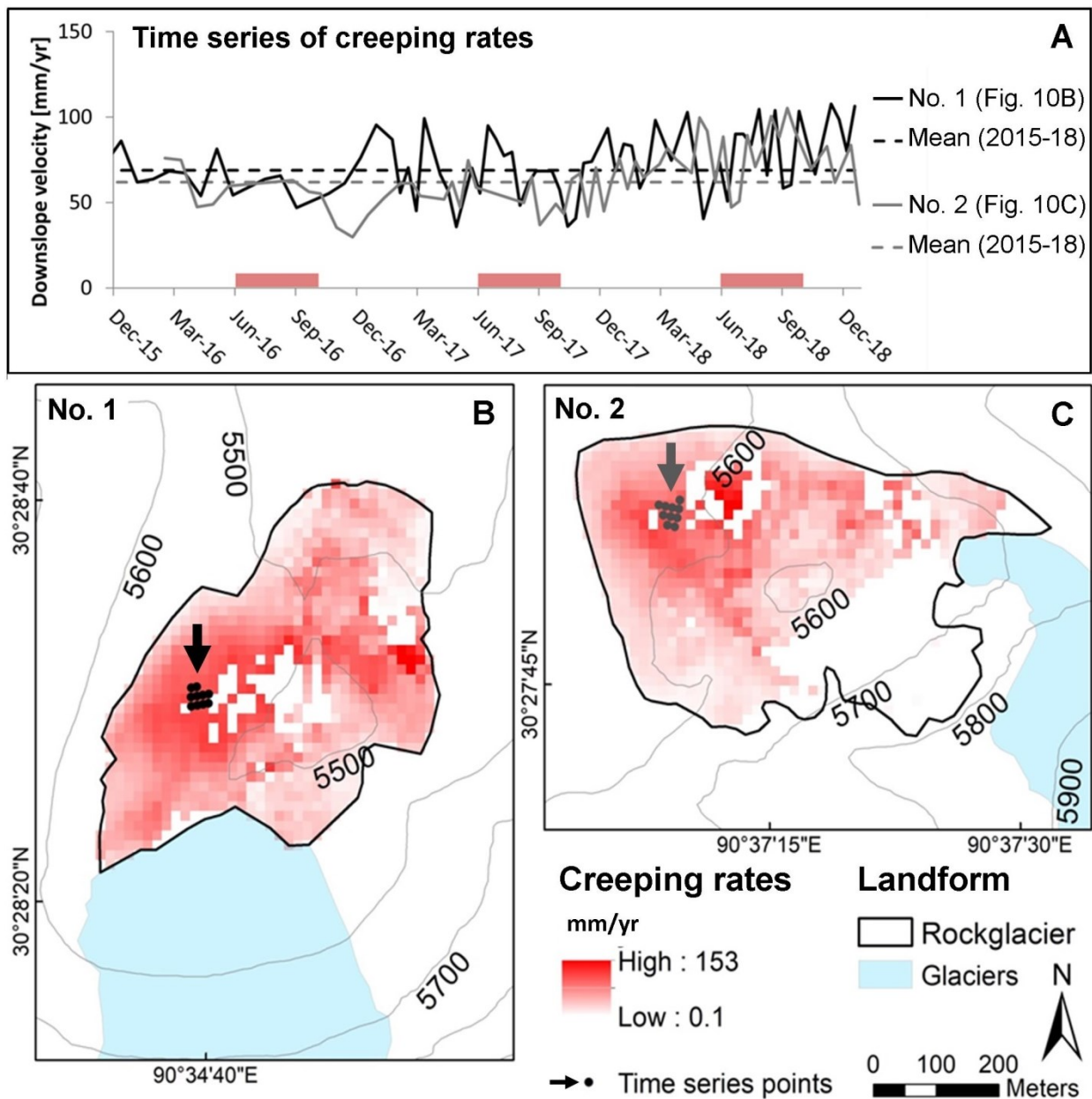
Figure 10: A: Summer months with air temperatures >0^{\circ}\text{C} (according to Zhang et al., 2013) are shown in red. Time series represent the moving average of the 10 nearest values in time based on the median of time series points, located in B (black dots) and C (grey dots). Black time series (rockglacier No. 1 in B) is based on ascending data and grey time series (rockglacier No. 2 in C) on descending data.
