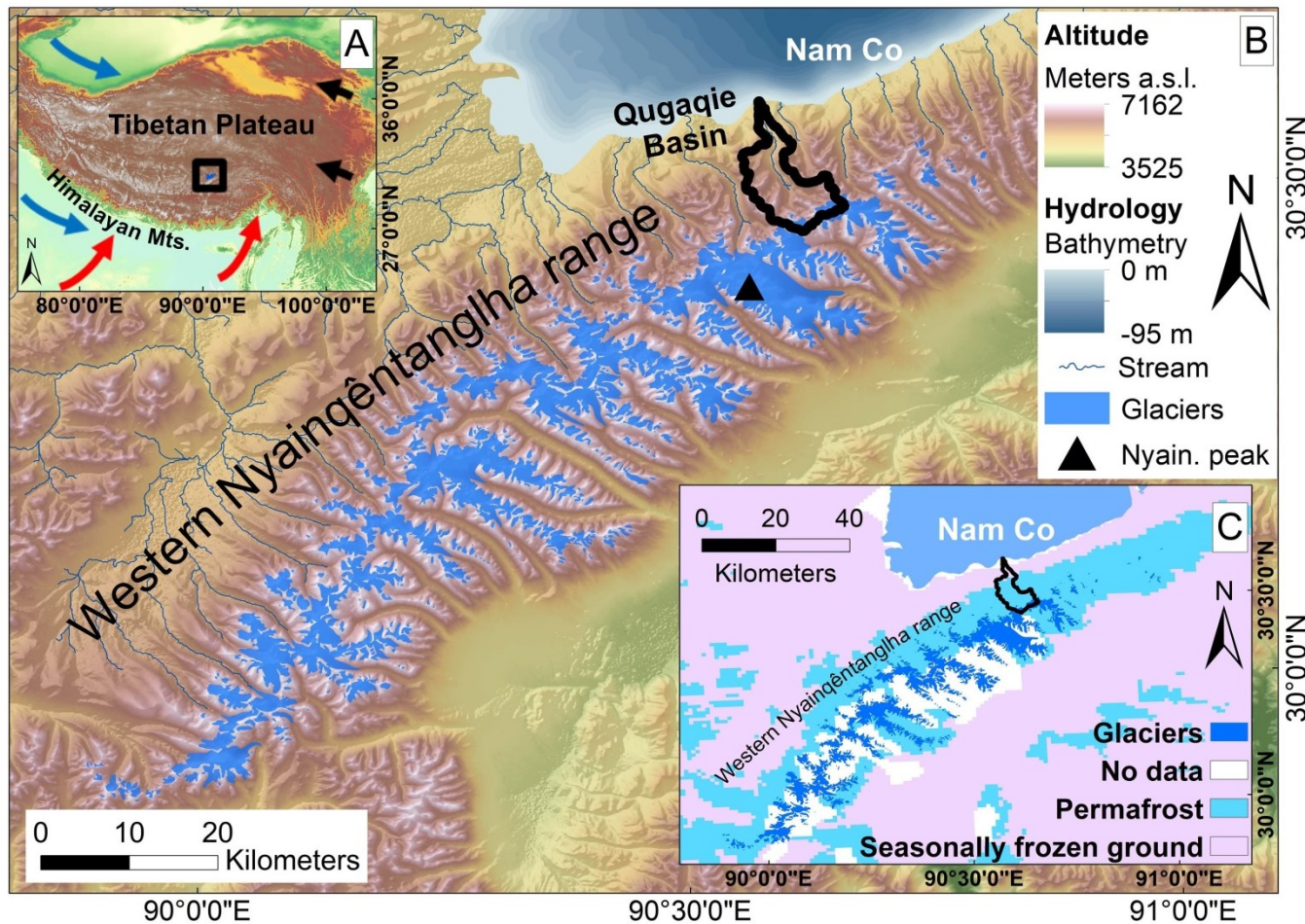
130 Figure 1: A: Location of the study area within the Tibetan plateau (TP) (Background on SRTM DEM v4; Jarvis et al., 2008). Different wind systems influencing climate of the TP are shown by blue (Westerlies), red (Indian Summer Monsoon) and black (East Asian Monsoon) arrows based on Yao et al. (2012). B: Overview map of the Nam Co catchment with the altitude colors and the study area of the Qugaqie catchment (thick black lines). Note the greater glacier extents on the south-oriented mountain range. Bathymetric data originated from (Wang et al., 2009) (Hillshade and DEM background based on SRTM DEM v4; Jarvis et al., 2008). Glacier extents originated from the GLIMS database (Cogley et al., 2015; Guo et al., 2015; Liu and Guo, 2014). C: Permafrost distribution in the Western Nyainqêntanglha range based on Zou et al. (2017).
