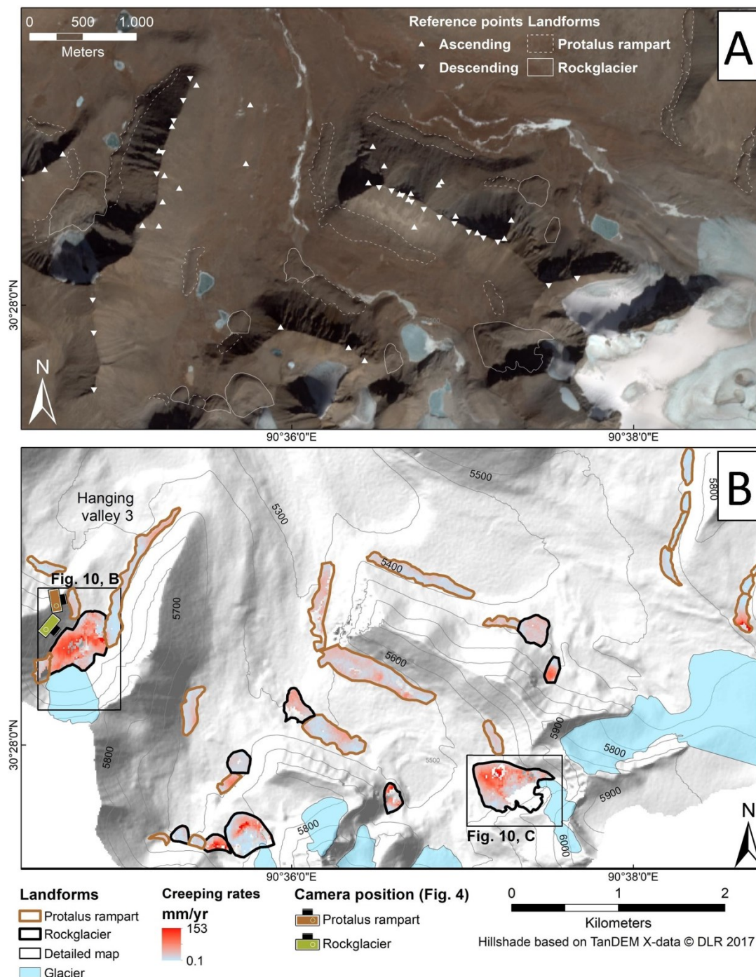
425 Figure 9: A: Sentinel II satellite image, recorded 30-01-2018. Triangles indicate stable reference points. Dashed lines indicate the outlines of the periglacial landforms. B: Creeping rates from periglacial landforms move in slope direction over the observation period 2015 - 2018. The Black rectangles mark the location of the two fastest rockglaciers in Figure 10. The Camera positions correspond to the Photographs in Figure 4.
