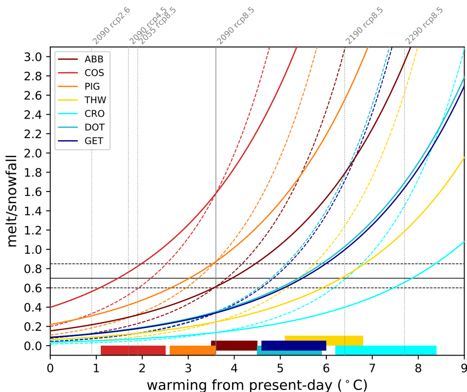
Figure 12. Extrapolated melt-to-snowfall ratio as a function of warming with respect to present-day (solid lines correspond to Eq. 2 and dashed lines to Eq. 3). The values obtained through our simulations correspond to the intersections with the vertical solid grey line. The vertical dashed grey lines represent warming at other dates (the dates indicated above the lines are the central years of 20-year averages) and under alternative scenarios (RCP2.6 and RCP4.5). This warming is derived from Collins et al. (2013, their Tab. 12.2), assuming that the regional warming remains equal to global warming (supported by our results as well as Collins et al., 2013). The black horizontal lines indicate three indicative thresholds for widespread runoff: the future 0.60 ratio simulated at Abbot in 2080-2100 (which is the minimum ratio for which we detect significant runoff), the 0.70 ratio estimated by Pfeffer et al. (1991), and the 0.85 ratio for which more than 50% of the grid points experience runoff (Fig. 7). The warming range for which the extrapolations cross the 0.60 and 0.85 thresholds are indicated by the horizontal color bars at the bottom.
