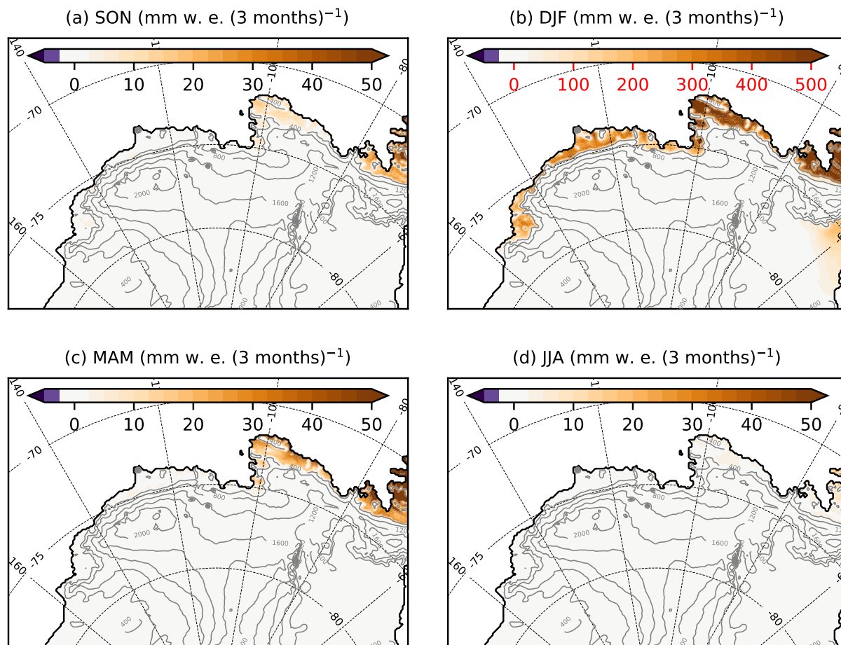
Figure 6. Changes in seasonal mean melt rates (future minus present). The colour-bar labels in panel (b) are shown in red to emphasise the different range compared to other panels. The ice-sheet topography is shown in grey (contours every 400 m).
