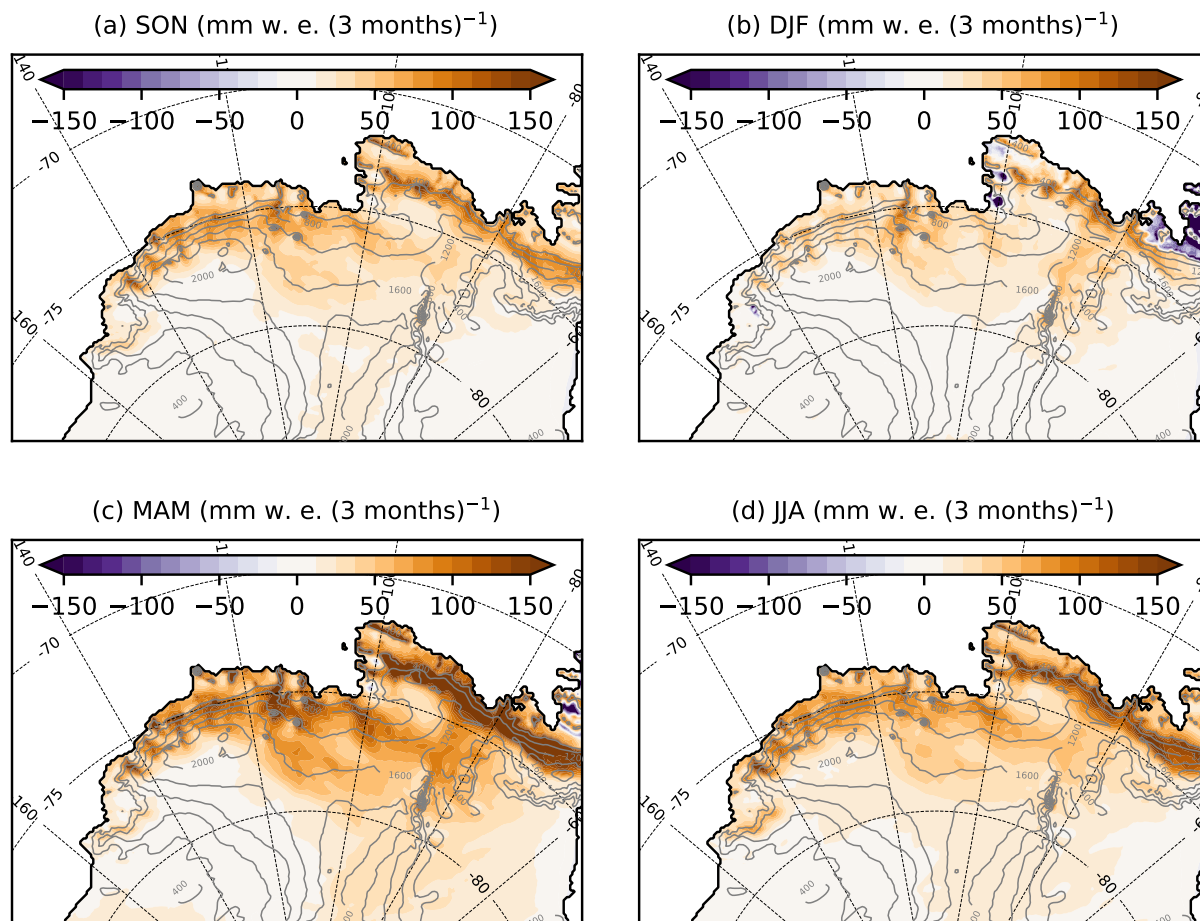
Figure 4. Changes in mean seasonal SMB (future minus present). The ice-sheet topography is shown in grey (contours every 400 m).
