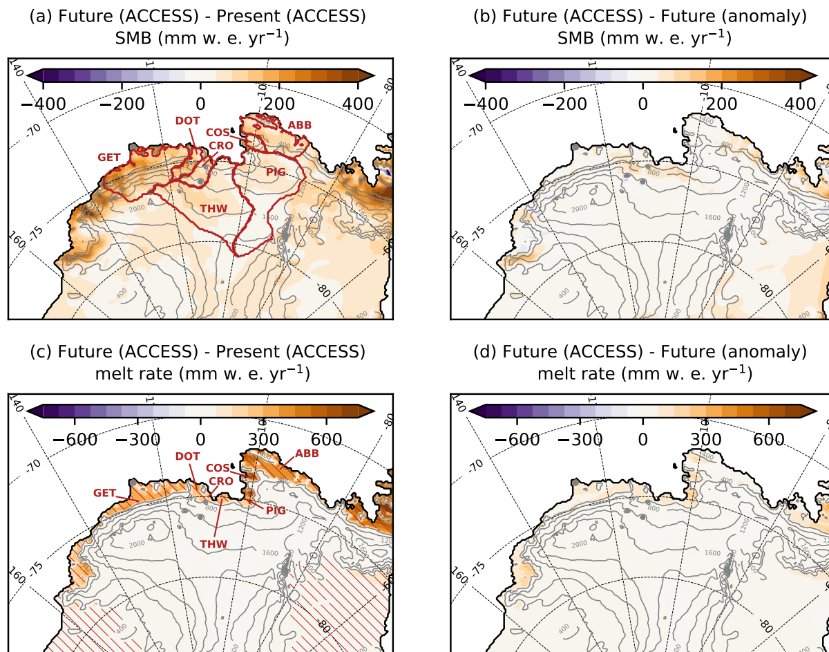
Figure 10. (a) SMB anomaly (2080-2100 minus 1989-2009) in ACCESS-1.3 directly downscaled by MAR (i.e. true changes). (b) Difference between the true future , from the direct downscaling of ACCESS-1.3, and the projected future , from the anomaly method. (c-d) Same as (a-b) but for melt rates instead of SMB. The dark red contours in the upper-left panel indicate individual glacial drainage basins (GETz, DOTson, CROsson, THWates, Pine Island Glacier, COSgrove, and ABBot). Red hatching in the lower panels indicate ice shelves. The ice-sheet topography is shown in grey (contours every 400 m).
