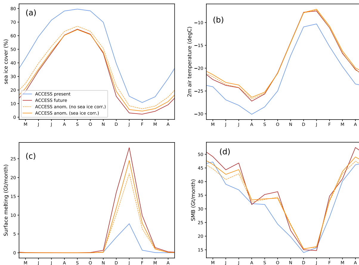
Figure 9. Mean 21-year seasonal cycle of: (a) domain-averaged sea-ice concentration, (b) 2 m air temperature, (c) surface melting and (d) SMB, with (b-d) integrated over the seven glacial drainage basins from Getz to Abbot (including both ice shelf and grounded ice). The blue and dark-red lines correspond to the present and true future based on ACCESS-1.3, respectively. The orange lines represent the results of the projected future , applied with (solid) and without (dashed) sea-ice iterative correction (see section 2).
