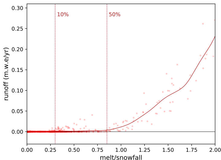
Figure 7. Runoff vs melt-to-snowfall ratio in the future simulation. Each circle represents the climatological annual mean at a grid point within the seven glacial drainage basins. The solid curve is a Gaussian kernel density estimate with a standard deviation of 0.1 melt-to-snowfall ratio. The vertical dashed lines indicate the limit above which more than 10% and 50% of the points experience a runoff greater than 1 mm w. e. yr -1 .
