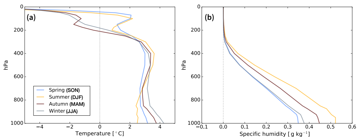
Figure 1. (a) temperature and (b) specific humidity vertical profiles of the CMIP5-MMM anomaly (2080-2100 minus 1989-2009) that is added to ERA-interim, here spatially-averaged over West Antarctica ( 60\text{--}85^{\circ}\text{S} , 170\text{--}40^{\circ}\text{W} ).
