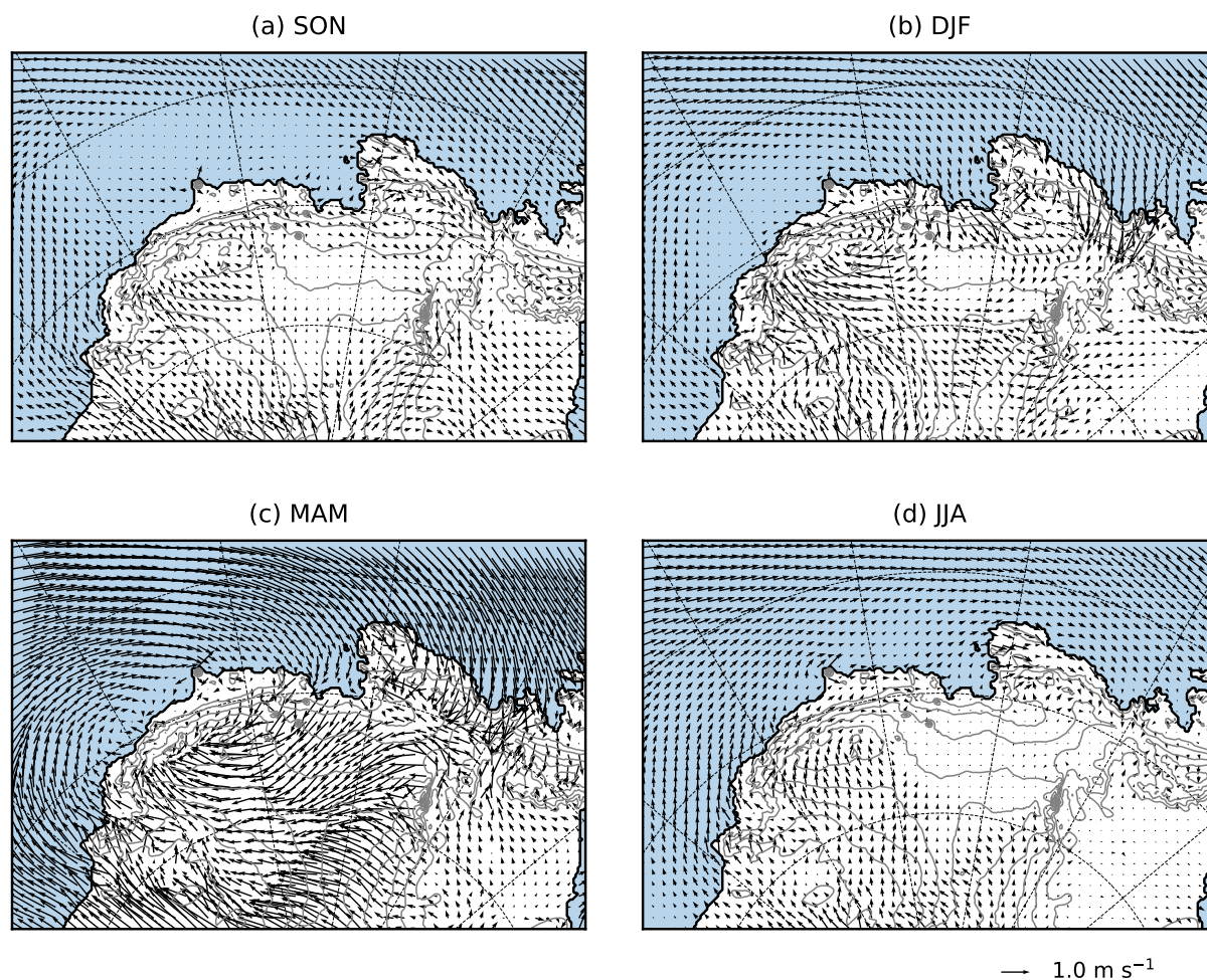
Figure 5. Changes in mean seasonal 10 m winds (future minus present). The open ocean is in light blue and the ice-sheet topography is shown in grey (contours every 400 m).
