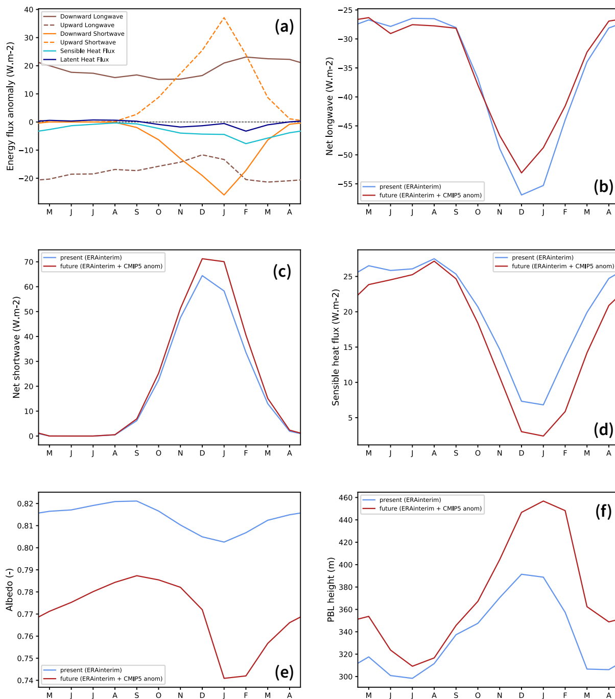
Figure 8. (a) Seasonal cycle of the anomaly (future minus present) in energy fluxes received by the ice-shelf surface (averaged over the seven major ice shelves from Getz to Abbot; positive if received by the surface). Present and future (b) net longwave radiative, (c) net shortwave radiative, and (d) sensible heat fluxes received by the ice-shelf surface. Mean present and future (e) albedo and (f) planetary-boundary-layer (PBL) height averaged over the seven major ice shelves from Getz to Abbot. The PBL height is calculated online in MAR from the vertical profile of horizontal turbulent kinetic energy.
