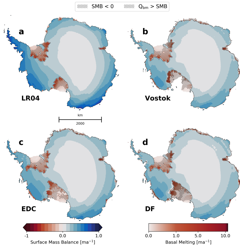
Figure 8. Surface Mass Balance (SMB, ma^{-1} ) for the grounded ice and basal melting ( Q_{bm} , ma^{-1} ) for the ice shelves for the CFEN simulations at 415 ka. Hatched areas show where basal melting dominates over surface mass balance and where surface mass balance is negative (i.e., where surface ablation occurs).
