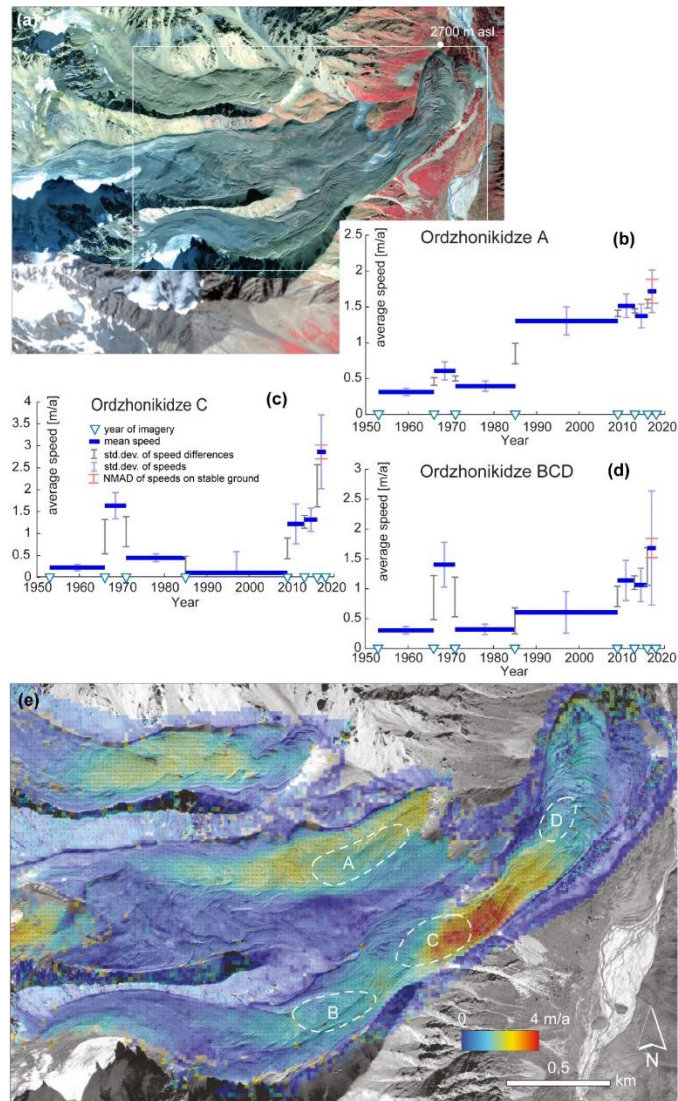
Figure 6: Velocities and speed variations across the Ordzhonikidze rock glacier system. (a) Overview image; GeoEye image (© Maxar) of 6 Oct 2013 in near-infrared false colour, with the southernmost part from a Planet image of 7 Sep 2016. (b-d) Average time series of speeds for clusters of points (zones A-D; white dashed outline in panel e). Error bars give standard deviations of speeds within the point clusters (blue), standard deviations of speed differences within the measurement periods (grey), and the NMAD of stable ground offsets (red, 2016-2018 only) in m/a. Blue triangles on the time axis indicate years of imagery used. (e) Colour-coded velocity field with vectors superimposed from image matching between 2016 and 2018 high-resolution satellite images (for exact dates and sensors see Table S2). Background image: GeoEye, 6 Oct 2013 (© Maxar).
