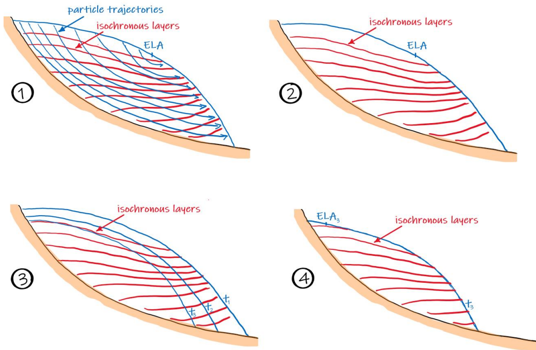
Fig. 2. In (1) we see the particle trajectories (blue) and the associated isochrones (red), emerging below the ELA; in (2) the trajectories have been removed to show only the isochrones; (3) shows subsequent
