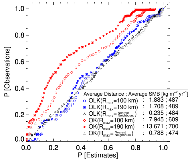
Figure 7. PP-plots between SMB observations and estimates based on OK and OLK interpolation methods for varying thresholds of their maximum distance R_{\text{max}} . The dashed 1:1 line indicates the complete PP-agreement between observations and estimates. Average PP-distances (see main text for definition) and SMB values are shown in the legend.
