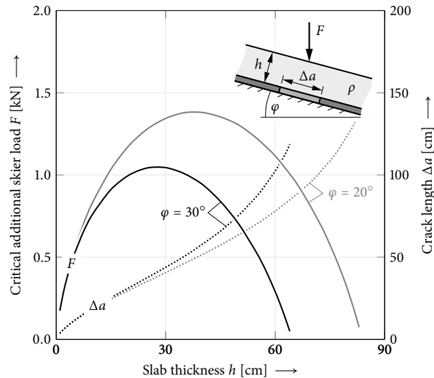
Figure 6. Critical loading of a snowpack without assumed defects and the size of initiated anticrack as a function of slab thickness. Thicker slabs transfer concentrated loads more uniformly allowing for larger point loads. Above a certain thickness, failure is dominated by the slab’s own weight reducing admissible additional loads until self-release occurs. The finite anticrack length increases continuously with increasing slab thickness.
