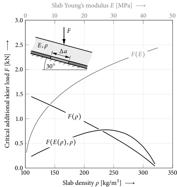
Figure 7. Effect of slab density \rho on critical additional skier loading F of a defect-free snowpack and the corresponding length of the initiated crack \Delta a . If the slab's Young's modulus is independent of slab density the increasing slab weight reduces the critical skier loading. A density-dependent Young's modulus according to Eq. (21) stiffens denser slabs which initially dominates failure and increases the critical skier load. Above a certain threshold, the weight gain becomes dominant and the critical skier loads reduces distinctly. The size of the initiated cracks \Delta a increases with slab density.
