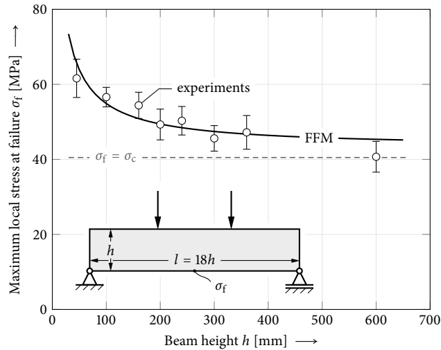
Figure 1. Size effect of wood beams in 299 self-similar four-point bending experiments. Experimental results reported by Fonselius (1997) are given as mean and standard deviation. Width of the beam is always b = 45 mm. Strength-of-materials solution (dashed) and finite fracture mechanics (FFM) prediction (solid) are shown.
