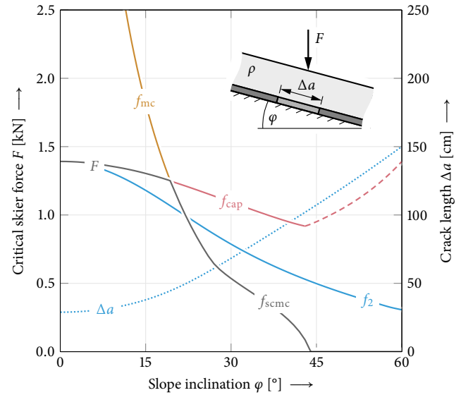
Figure 9. Comparison of mixed-mode stress criteria for a defect-free snowpack with slab thickness h = 20 \text{ cm} . The quadratic interaction criterion f_2 , the smooth capped Mohr-Coulomb criterion f_{scsmc} as well as its constituents f_{mc} and f_{cap} are shown.
