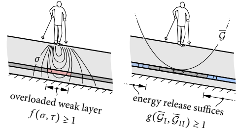
Figure 2. Coupled stress and energy criterion for the case of a skier loaded snowpack. On the left the condition of a locally overloaded weak layer and on the right the second condition of sufficient energy release rate are shown. The stress condition has the effect of an upper bound on possible nucleated cracks. Whereas the energy condition provides a lower bound on the crack lengths as short cracks do not release sufficient energy.
