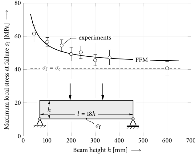
Figure 1. Size effect of wood beams in 299 self-similar four-point bending experiments. Experimental results reported by Fonselius (1997) are given as mean and standard deviation. Out-of-plane width of the beams is always b = 45 mm. Strength-of-materials solution (dashed) and finite fracture mechanics (FFM) prediction (solid) are shown.
