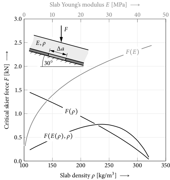
Figure 7. Effect of slab density \rho on critical skier force F of a defect-free snowpack and the corresponding length of the initiated crack \Delta a . If the slab's Young's modulus is independent of slab density, curve F(\rho) , the increasing slab weight reduces the critical skier force. A density-dependent Young's modulus according to Eq. (22), curve F(E(\rho), \rho) , stiffens denser slabs, which initially dominates failure and increases the critical skier load. Above a certain threshold, the weight gain becomes dominant and the critical skier force reduces distinctly.
