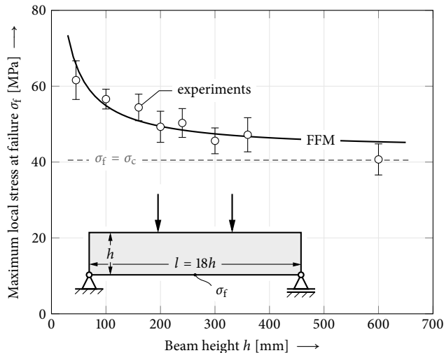
Figure 1. Size effect of wood beams in 299 self-similar four-point bending experiments. Experimental results reported by Fonselius (1997) are given as mean and standard deviation. Out-of-plane width of the beams is always b = 45 mm. Strength-of-materials solution (dashed) and finite fracture mechanics (FFM) prediction (solid) are shown.
